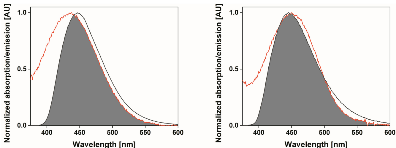
Figure 5. Left: The spectral overlap between 2CNqA emission (black line; \lambda_{\text{Exc}} = 355 nm) and qA_{\text{nitro}} absorption (red line) in dsDNA. Measured in 13 mM sodium phosphate buffer, 100 mM NaCl, pH 7.5 at RT. Right: The spectral overlap between 2CNqA emission (black line; \lambda_{\text{Exc}} = 354 nm) and tC_{\text{nitro}} absorption (red line) in dsRNA. Measured in 10 mM sodium phosphate buffer, 100 mM NaCl, 1.0 mM EDTA, pH 7.4 at RT. For both DNA and RNA, the spectra are normalised at their long-wavelength maxima.
