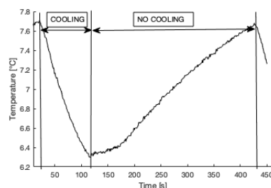
Figure 2: Temperature development in a refrigerated display cabinet during maximum cooling followed by no active cooling. Results are from a pilot experiment by the authors.
