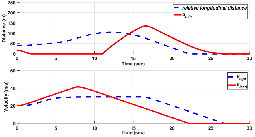
Figure 6: The relative and safe distance, and the vehicle velocities for a_{lead0} = 3 and a_{lead1} = -3 . At around 14 s the relative distance between the vehicles becomes less than d_{min} , and a collision occurs at around 22 s.
