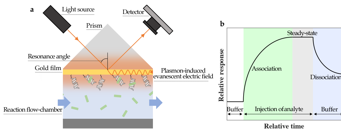
Figure 17: (a) Schematic illustration of a typical SPR setup. Upon binding of analyte (green) to the substrate (immobilized DNA) the local refractive index will change, which is monitored by measuring the resonance angle with time. (b) A characteristic SPR sensogram is generated, from which the binding kinetics can be obtained. The relative response reflects variations in the resonance angle and in turn the interaction between substrate and analyte with time. The association event is followed by a steady-state phase, where equilibrium is reached. Post-injection buffer flow will allow the analyte to dissociate from the substrate, resulting in a declining relative response.
