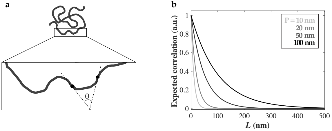
Figure 2: (a) A schematic illustration of a coiled polymer in accordance with the worm-like chain model, where the angular difference ( \theta ) between tangents along the contour indicates the flexibility. (b) The expected relative correlation between tangents, given by the average cosine of \theta at given values for the persistence length ( P ), calculated from Eq.1. The expected correlation decreases exponentially with increasing distance ( L ).
