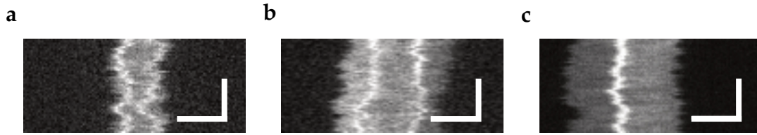
Figure 34: (a) Kymographs of a single circularized \lambda -DNA-CtIP wt complex with two mobile local condensates along the extension. (b) A higher-order complex of two concatemeric \lambda -DNA molecules, subsequently circularized in the presence of CtIP wt , harboring two mobile local condensates. (c) Two circularized \lambda -DNA-CtIP wt complexes joined through a central, static condensate. Vertical and horizontal scale bars correspond to 3 s and 3 \mu m, respectively.
