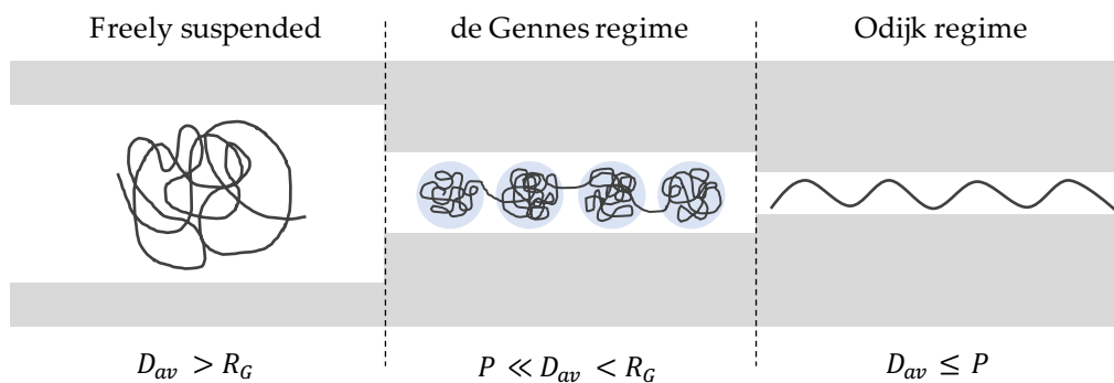
Figure 4: The behavior of a polymer under different degrees of confinement in a channel. The coiled structure will be retained at channel dimensions ( D_{av} ) larger than the radius of gyration ( R_G ). At smaller dimensions, the extended polymer can be described as a series of non-interacting units, according to the model proposed by de Gennes. At dimensions smaller than the persistence length ( P ), the polymer will enter into the Odijk regime.
