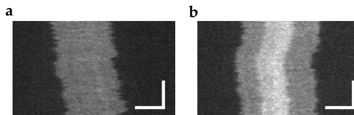
Figure 21: (a) Kymograph of a \lambda -DNA molecule, labelled with YOYO-1. Upon confinement in a nanofluidic channel, the molecule will stretch to accommodate. For this particular molecule the total extension corresponds to approximately 59% of the contour length of bare \lambda -DNA. (b) Kymograph of a higher-order DNA-protein complex, formed in the presence of the bacterial Ku. The central bright patch reflects the local increase of YOYO-1 as a result of two overlapping \lambda -DNA molecules. The vertical and horizontal scale bars correspond to 3 s and 5 \mu m, respectively.
