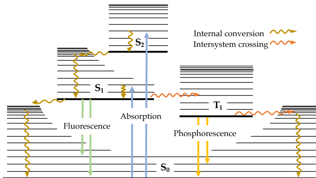
Figure 13: Electronic transitions visualized in a Jablonski diagram. Upon excitation (straight blue arrows) from the ground electronic level ( S_0 ) electrons will occupy different vibrational levels in the excited state. The molecule will lower its energy mainly through non-radiative processes, such as internal conversion and intersystem crossing (undulating arrows), to finally relax back to S_0 . Relaxation can also occur through fluorescence and phosphorescence, which are radiative processes (straight yellow and green arrows, respectively), where photons are emitted upon deactivation of the electrons from the excited singlet ( S_1 ) or triplet ( T_1 ) levels to S_0 , respectively.
