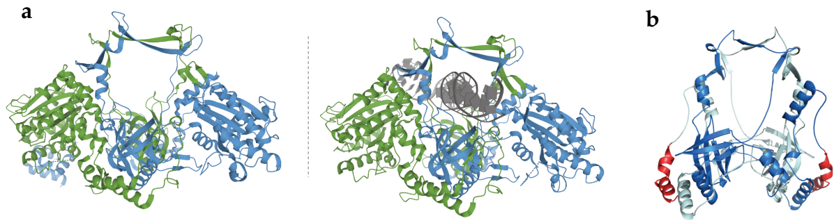
Figure 12: (a) Structure of the human Ku70/80 heterodimer in the absence (left) and presence (right) of DNA (grey). The Ku70 and Ku80 subunits are visualized in blue and green, respectively. The images were derived from data submitted to Protein Data Bank (PDB: 1JEQ and 1JEY) 106 . (b) Structural prediction of the bacterial Ku homodimer, where the two identical subunits are visualized in different shades of blue. The protruding C-terminal regions are highlighted in red. The structure was generated by comparative modeling, using the eukaryotic Ku70/80 heterodimer in (a) as template.
