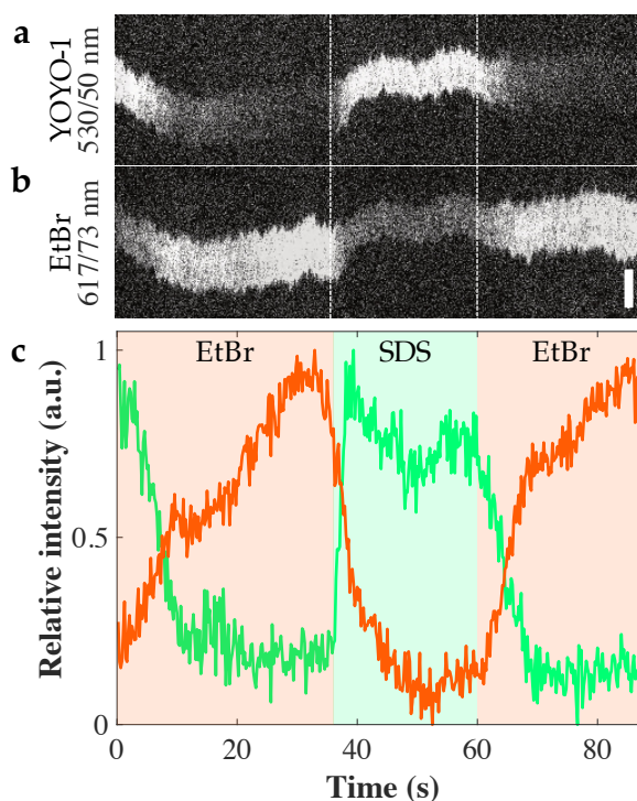
Figure 27: Sequential addition of EtBr and SDS to a YOYO-1 stained \lambda -DNA molecule. The kymographs show the fluorescence emission of (a) YOYO-1 and (b) EtBr over time, using only blue light of 470/24 nm for excitation. (c) Relative fluorescence intensities of YOYO-1 (green) and EtBr (orange) with time, respectively. The background color shades represent the timepoints, at which transitions are detected in the emission pattern upon change of analyte between EtBr (orange) and SDS (green). Scale bar corresponds to 5 \mu m.
