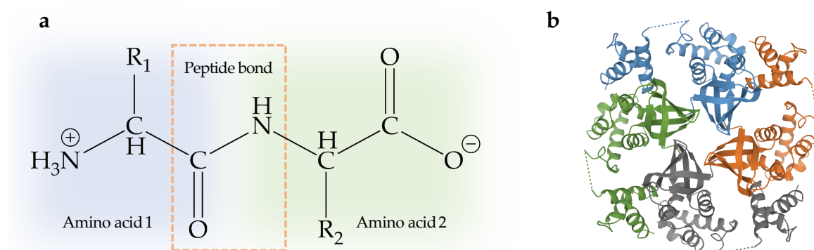
Figure 8: (a) Two amino acids linked through a peptide bond. (b) Quaternary structure of the Escherichia coli homotetrameric RuvA helicase, where each subunit is highlighted in a different color. The \alpha -helical structural motifs are mainly covering the outer surface, while \beta -sheets are hidden in the core of the protein complex. The image was derived from data submitted to Protein Data Bank (PDB: 1CUK) 51 .
