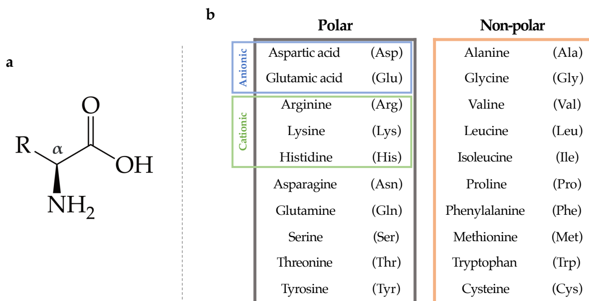
Figure 7: (a) Molecular structure of a generic amino acid. The \alpha -amine and \alpha -carboxyl groups along with the variable side chain, denoted as R, are connected to the \alpha -carbon atom. (b) Summary of amino acids, used in the protein synthesis, with the corresponding three-letter abbreviations. The overall polarity is determined by the variable side chain.
