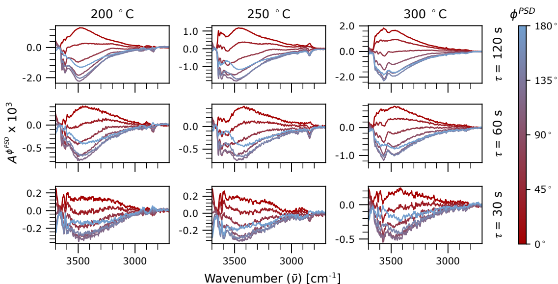
Figure 4. Phase resolved spectra in the 3800–2700 cm −1 region ( 0^\circ \leq \theta^{\text{PSD}} \leq 180^\circ ), showing responding hydroxyl and C–H vibrations.
