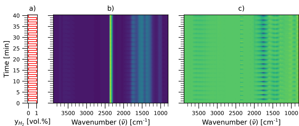
Figure 2. Modulation excitation spectroscopic measurement of CO 2 hydrogenation over a Rh/CeO 2 catalyst at 300 °C showing: (a) the imposed H 2 concentration stimulus with period \tau = 120 s; (b) collected background subtracted in situ infrared spectra; and (c) collected background subtracted in situ infrared difference spectra where the first spectrum was subtracted from each remaining spectrum in the full measured range 3900–800 cm -1 .
