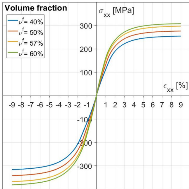
Fig. 8. Model predictions for different fiber volume fractions \nu^f . A specimen with the off-axis angle 45^\circ is considered.
