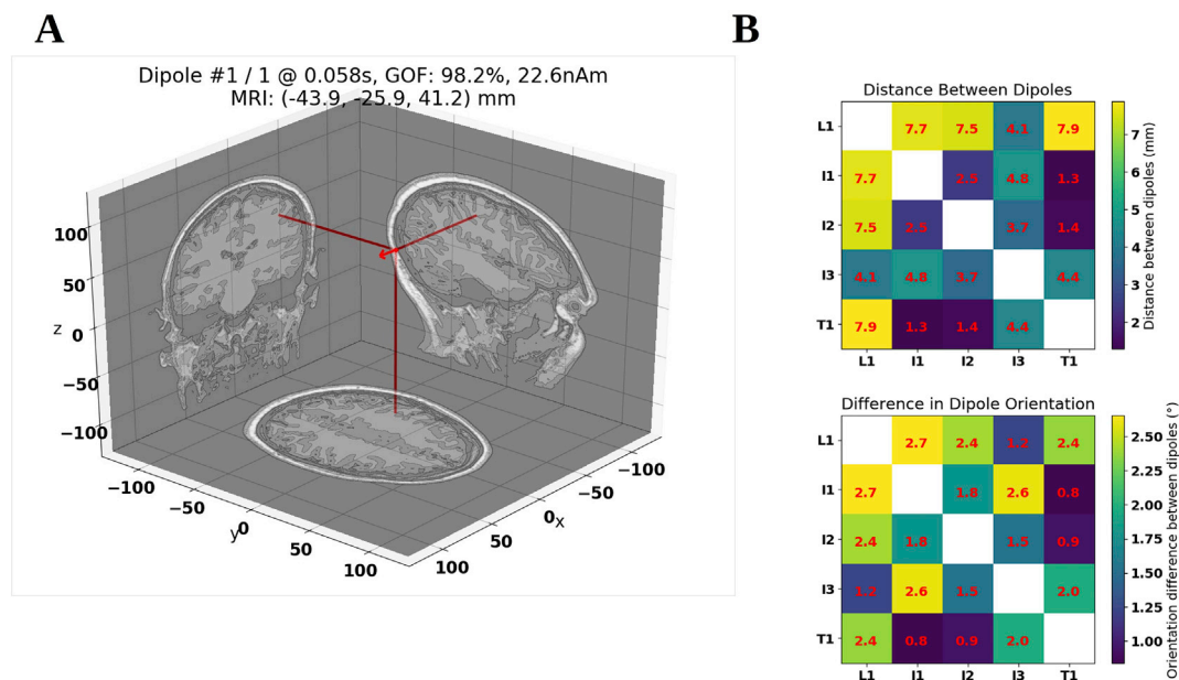
Fig. 3. Dipole fit and peak classifications for Subject 4: A : Position and orientation of fitted dipole of I1. The dipole was fitted to contralateral SI. B : Distances and orientation differences between fitted dipoles. L1 is the one furthest away from all other dipoles and it also shows the greatest orientation difference compared to the others.
