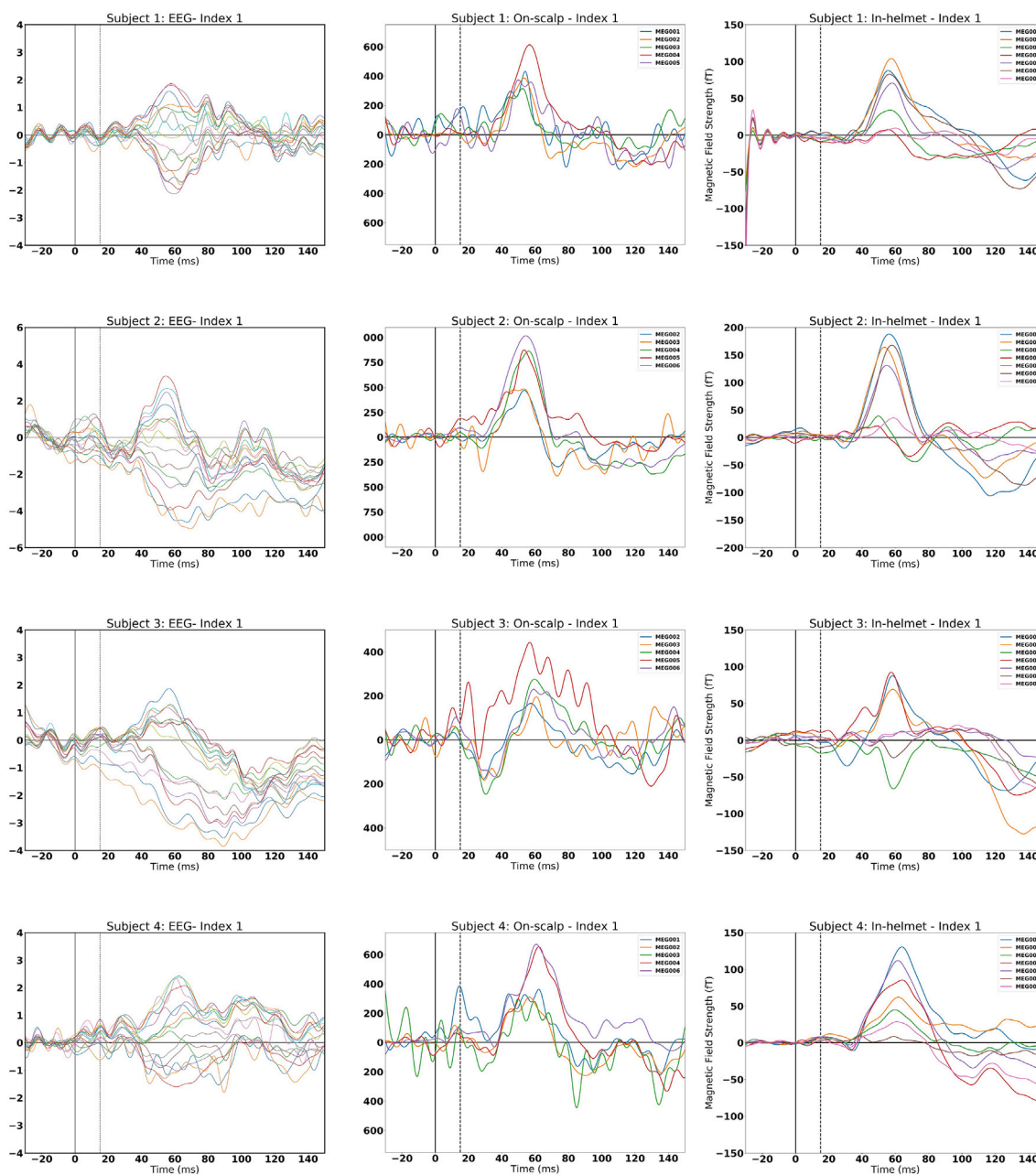
Fig. 5. Evoked responses for Index 1 for all subjects and all sensors. Left column is EEG, middle column is on-scalp and right column is in-helmet. Punctured line for all plots is at 15 ms. All subjects have at least one magnetometer showing a peak at 15 ms for the on-scalp recordings, whereas there are no clear peaks for the in-helmet recordings. See Supplementary Fig. 8 for the minimum recordings. A high-pass filter of 1 Hz has been applied to the EEG recordings.
