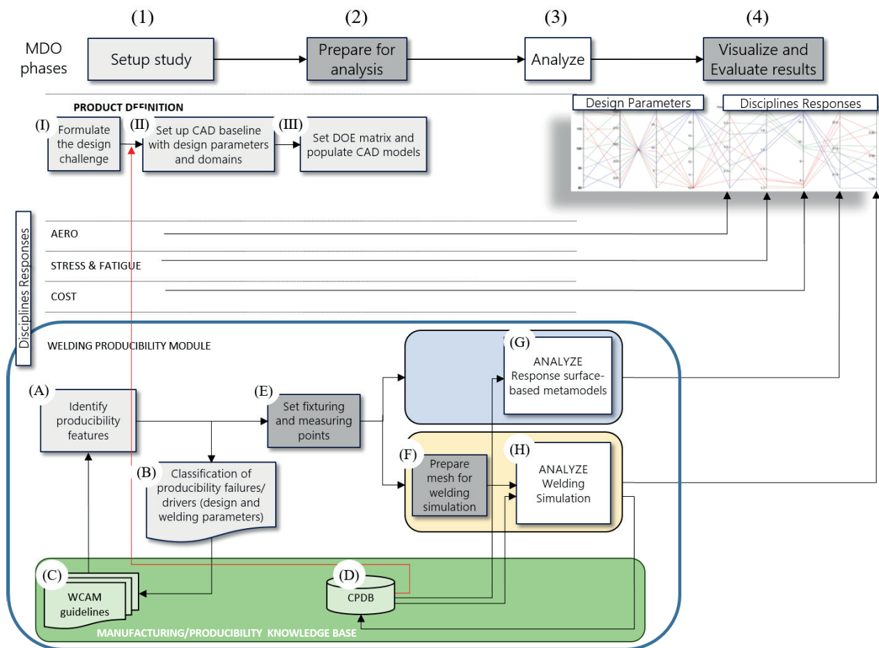
Figure 32 Producibility analysis module consisting of two analysis steps in a MDO enviroment
