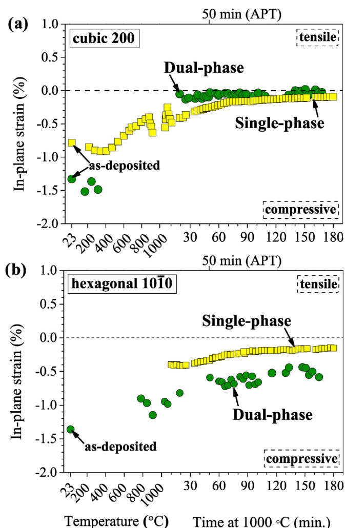
Fig. 9. Strain evolution during annealing: (a) in the cubic phase recorded using the 200 diffraction line and (b) in the hexagonal phase recorded using the 10 \bar{1}0 diffraction line.
