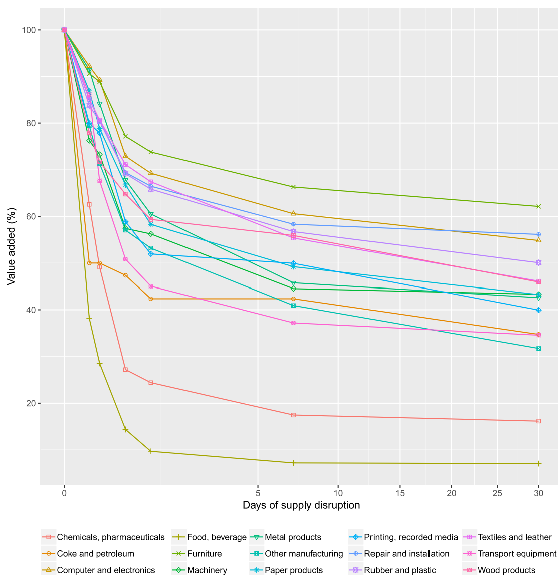
Figure 5.15 Maintained value added for the manufacturing sectors, expressed as a percentage of normal business activity during water supply disruptions of different durations.
