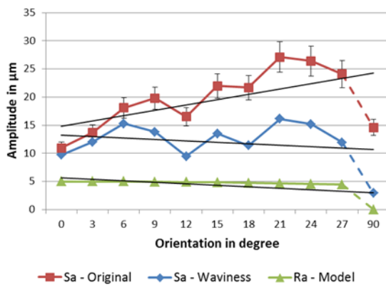
Figure 23. Average roughness curve
