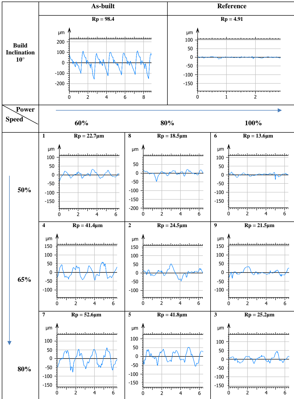
Figure 32. Profile measurements
