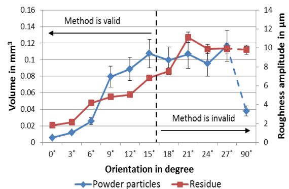
Figure 24. Volume curve of the powder particles and Sa of residue plotted against the build orientation.
