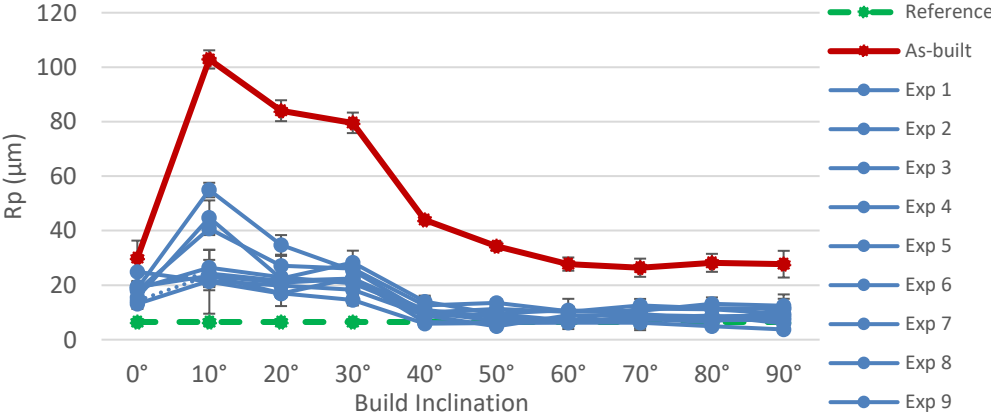
Figure 31. The maximum peak height of laser finished FDM surface at various build inclination along with as-built and reference injection molding measurements.
