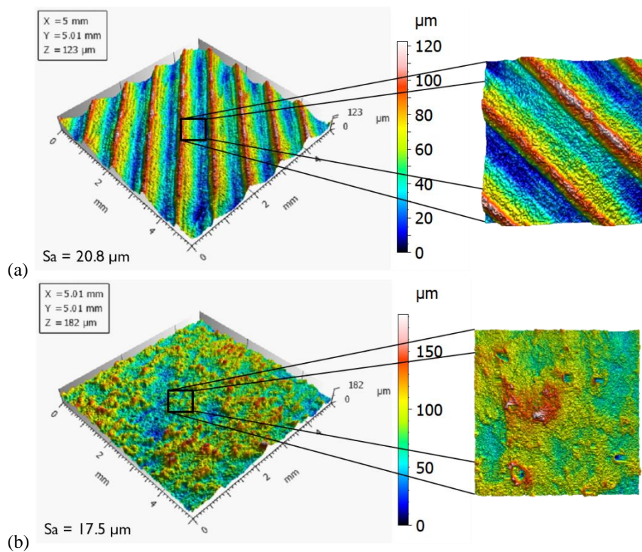
Figure 10. The 3D view of surface topography of FDM surfaces at 0° build inclination (a) as-built and (b) laser finished surface.
