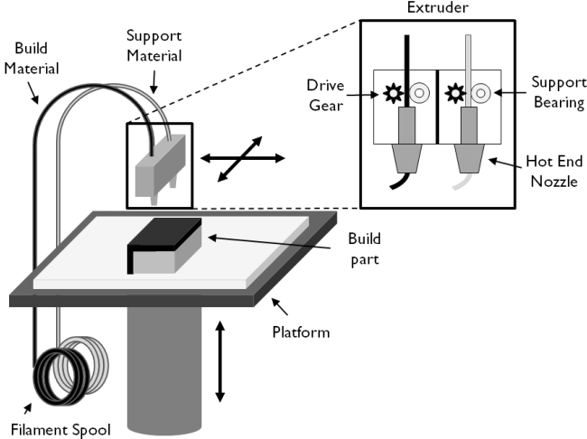
Figure 7. Illustration of the FDM process
