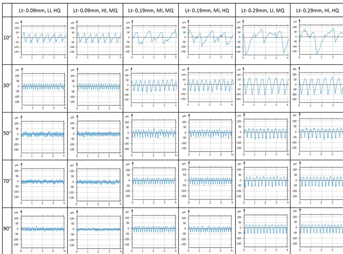
Figure 35. Roughness profile measurements
