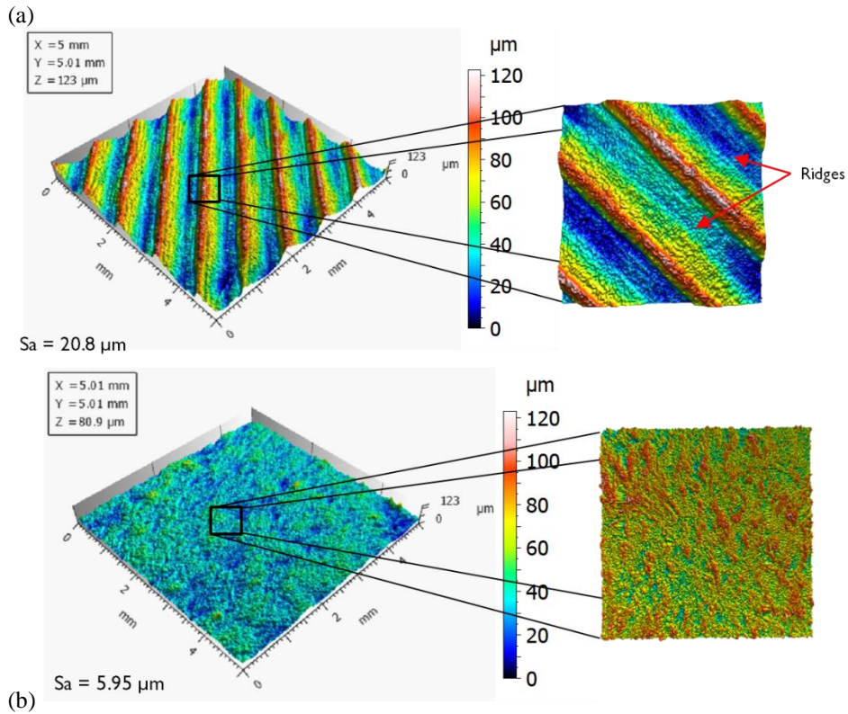
Figure 11. The 3D view of surface topography of FDM surfaces at 0^\circ build inclination (a) as-built and (b) Acetone-vapour finished surface.
