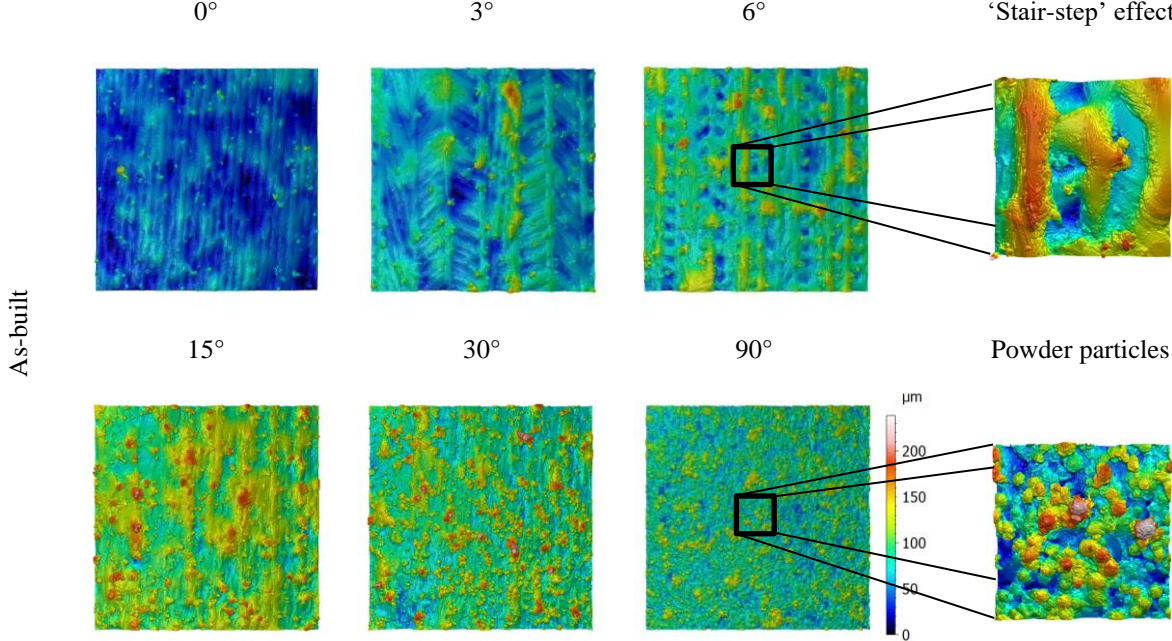
Figure 6. 3D topography view of as-built PBF-LB/M surfaces at various build inclinations. All surfaces have a measurement area of 2.5 mm×2.5 mm and the extracted surface has an area of 0.5 mm×0.5 mm.
