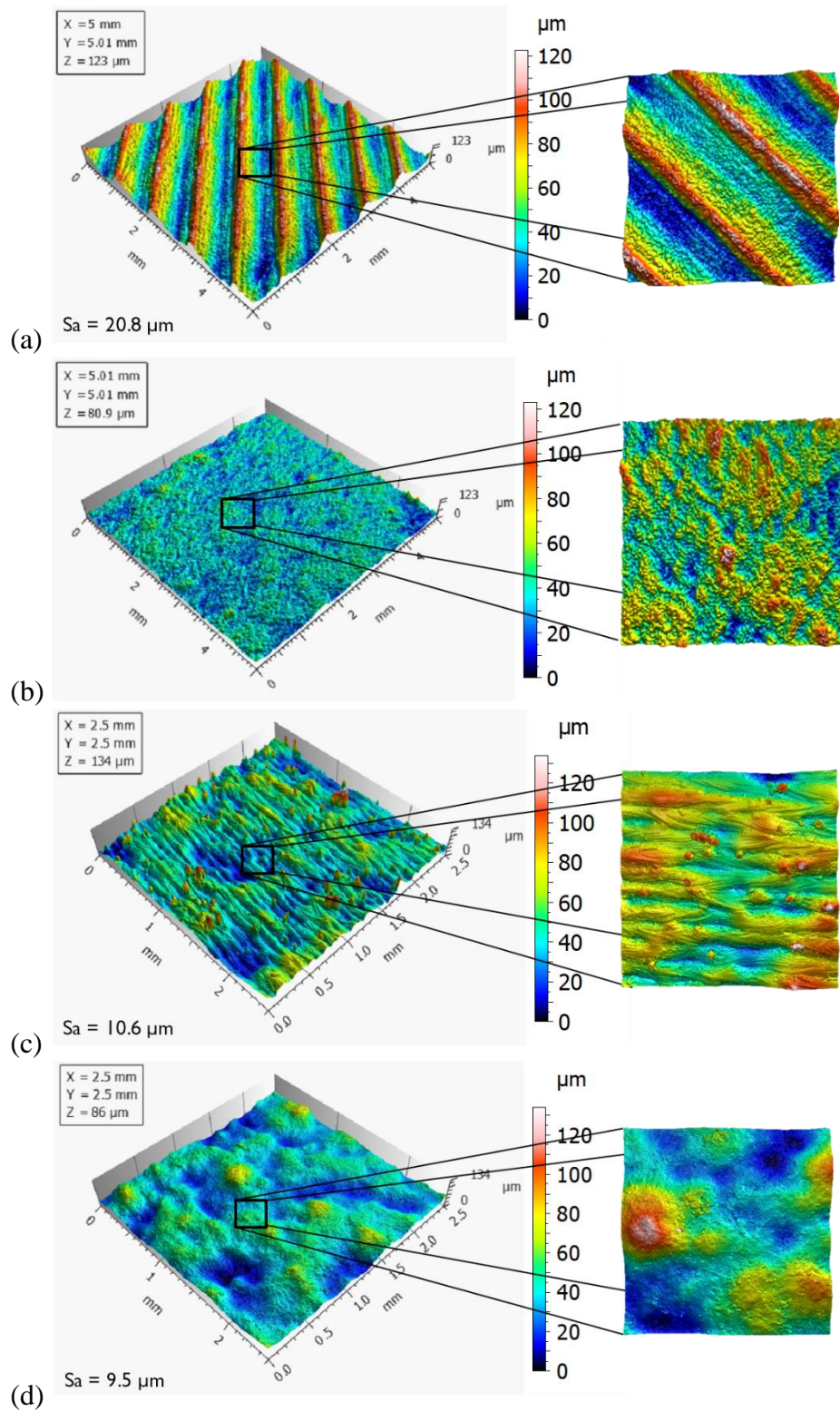
Figure 9. The 3D view of surface topography at 0^\circ build inclination (a) as-built FDM surface, (b) shot-blasted FDM surface; (c) as-built PBF-LB/M surface and (d) shot-blasted PBF-LB/M surface.
