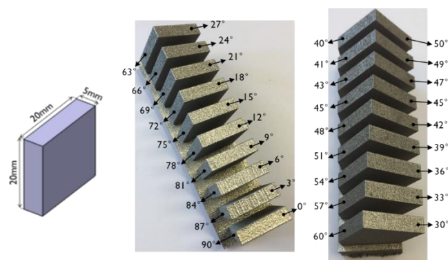
Figure 25. Truncheon artefact with varying build inclination.
