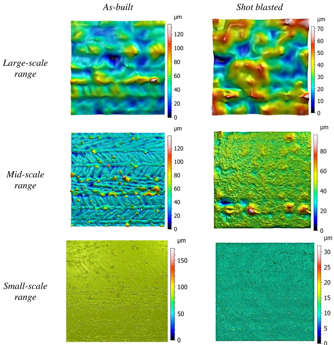
Figure 28. Filtered surface topography of as-built and shot blasted sample at 3^\circ build inclination for large, mid and small scale ranges. Measurement area was maintained at 2.5\text{mm} \times 2.5\text{mm} .
