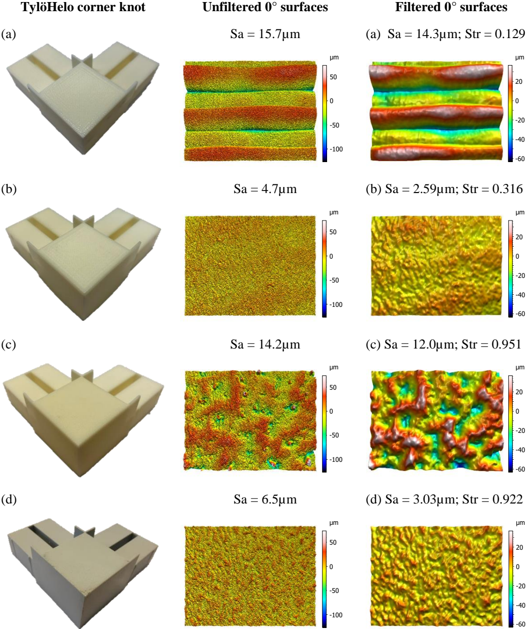
Figure 34. TylöHelo sauna corner knot with unfiltered and filtered surfaces (a) As-built FDM surface (b) Acetone + glass blasted surface (c) Laser + glass blasted surface (d) Reference injection molding surface. Measurement area of the captured surfaces is 2.5mm × 2.5mm.
