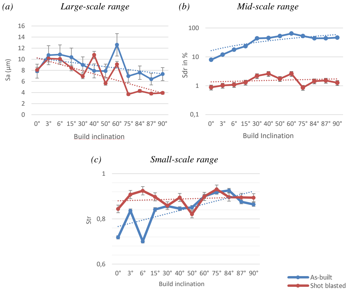
Figure 29. Variation of selected significant parameters with respect to build inclination in corresponding scale ranges.
