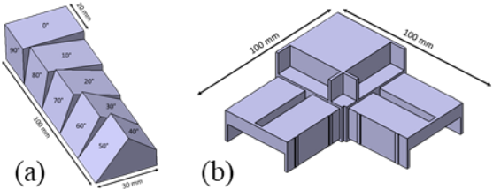
Figure 30. CAD models of (a) Truncheon artefact and (b) TylöHelö sauna corner knot.
