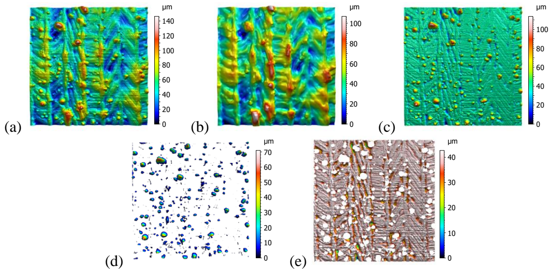
Figure 22. Isolation of powder particles and staircase effect by applying the Robust Gaussian filter. (a) Original surface (b) Waviness surface (c) Roughness surface (d) Powder particles (e) Residual surface. Measurement area of the captured surface is 2.5\text{mm} \times 2.5\text{mm} .
