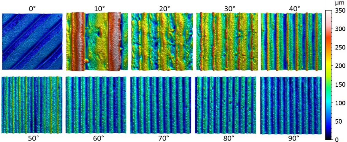
Figure 8. The 3D view of surface topography of the as-built FDM sample with varying build inclinations to show the stair-step effect. All surfaces have a measurement area of 2.5 mm×2.5 mm.
