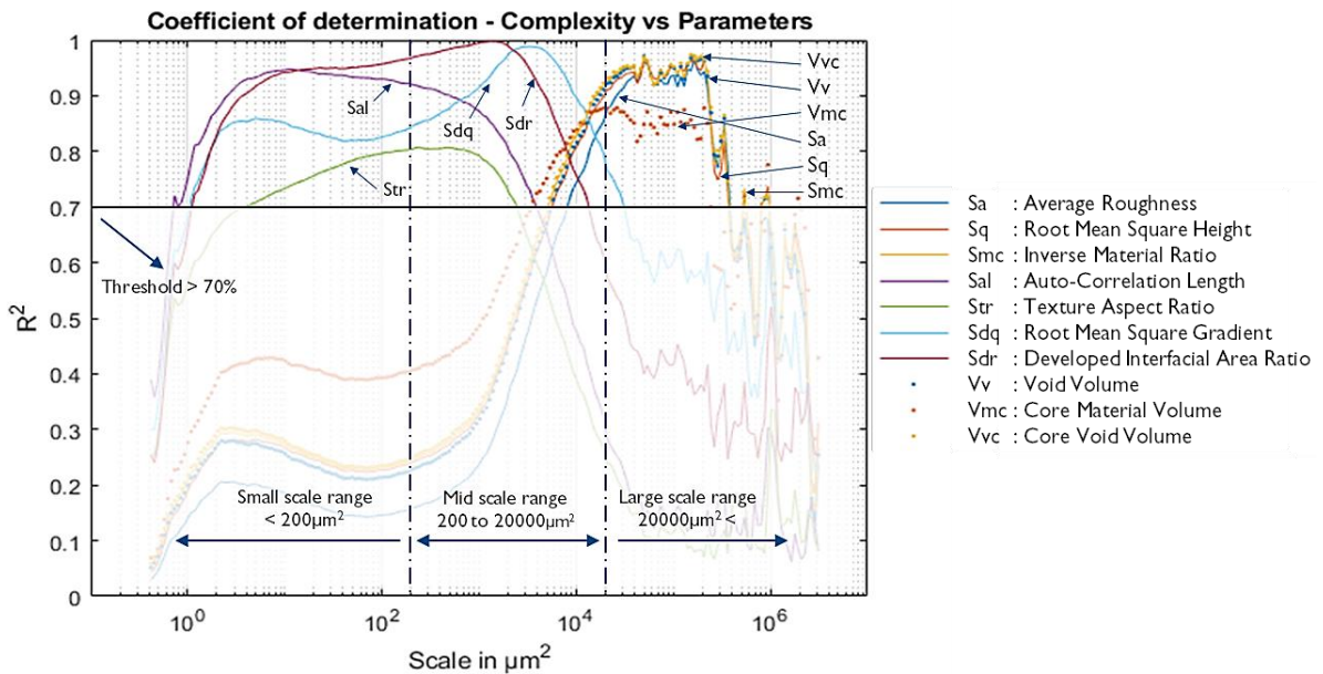
Figure 27. Coefficient of determination ( R^2 ) of significant parameters obtained by taking correlations between the complexity values and areal surface texture parameters at every scale.
