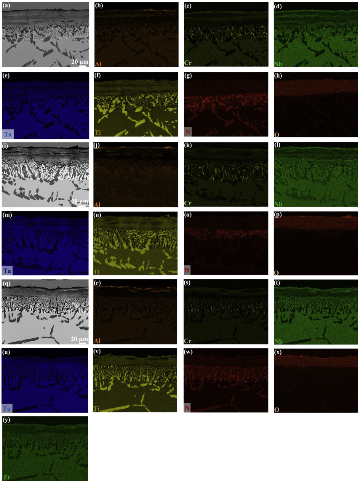
Fig. 7. Cross-sectional EDS elemental mapping of (b–h) Al_{0.5} , (j–p) Al_{0.75} , and (r–y) Al_{0.5}Zr_{0.01} specimens after 100 h of exposure at 1,100 °C. The corresponding cross-sectional microstructures given in (a), (i), and (q) are the same as those shown in Fig. 6.
