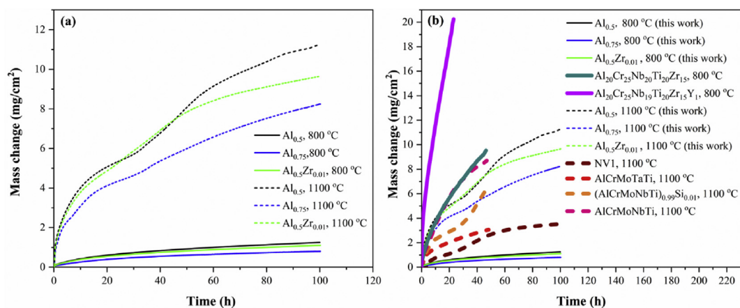
Fig. 2. (a) Specific mass change versus time plots for \text{Al}_{0.5} , \text{Al}_{0.75} , and \text{Al}_{0.5}\text{Zr}_{0.01} at 800 °C (solid lines) and 1,100 °C (dotted lines); (b) comparison of specific mass change versus time between studied RHEAs in this work and selected RHEAs from the literature.
