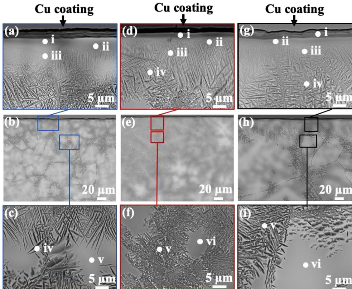
Fig. 4. Cross-sectional microstructures of (a–c) Al 0.5 , (d–f) Al 0.75 , and (g–i) Al 0.5 Zr 0.01 specimens after 100 h of exposure at 800 °C.
