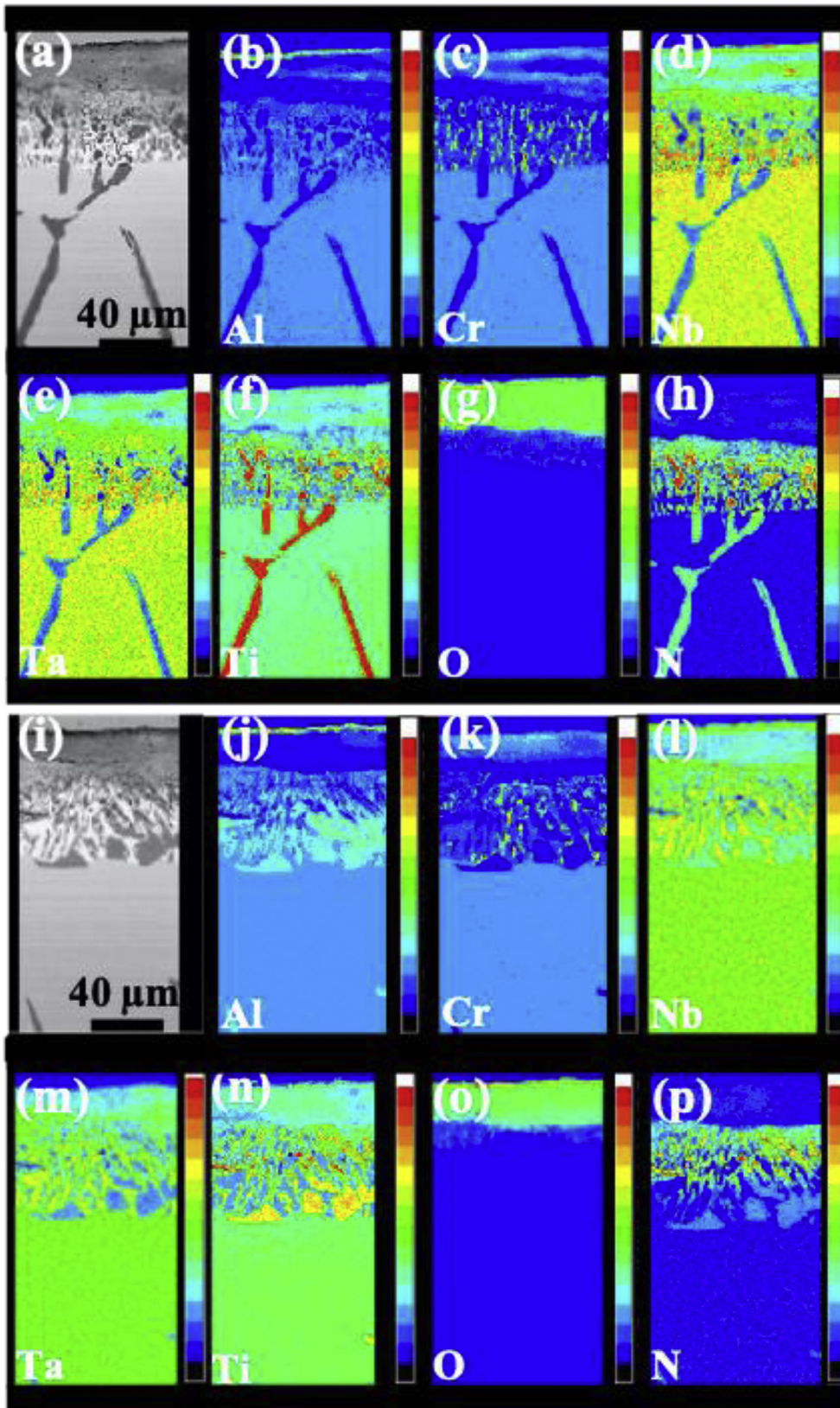
Fig. 8. Cross-sectional microstructures and EPMA elemental mapping of (a–h) Al_{0.5} and (i–p) Al_{0.75} specimens after 100 h of exposure at 1,100 °C.
