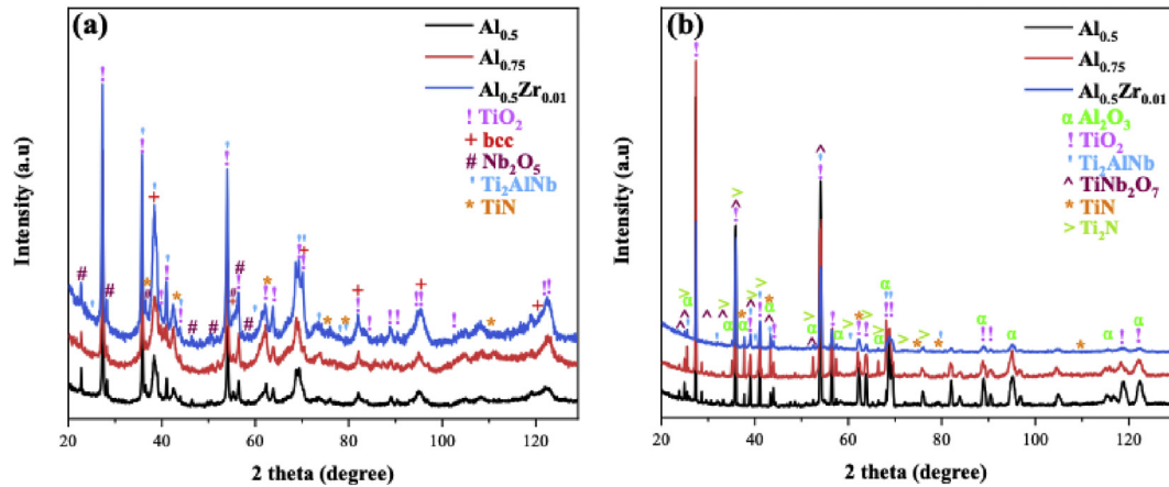
Fig. 3. XRD patterns of Al 0.5 , Al 0.75 , and Al 0.5 Zr 0.01 specimens after 100 h of exposure at (a) 800 °C and (b) 1,100 °C.
