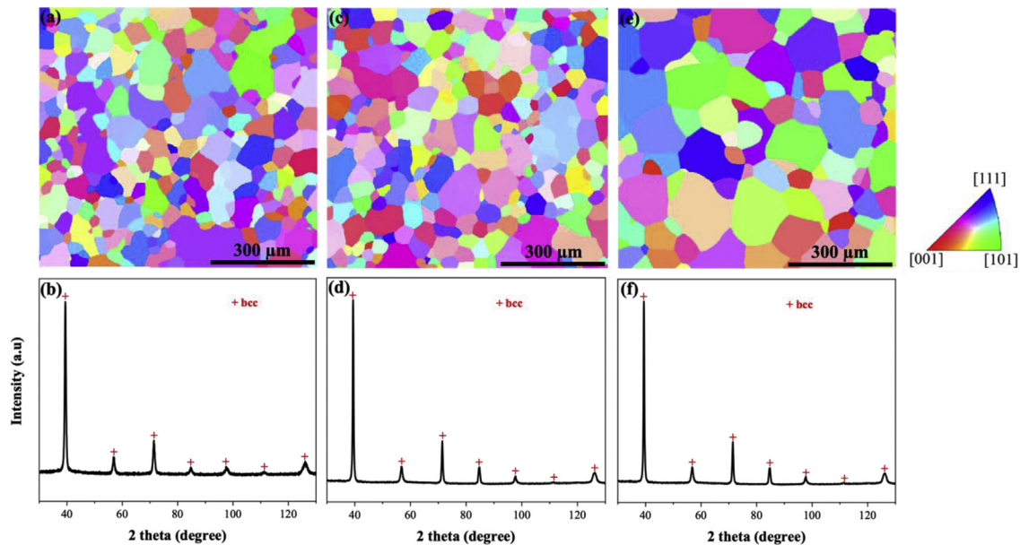
Fig. 1. EBSD IPF maps and their corresponding XRD patterns of the as-cast RHEAs. (a) and (b) are for \text{Al}_{0.5} , (c) and (d) are for \text{Al}_{0.75} , and (e) and (f) are for \text{Al}_{0.5}\text{Zr}_{0.01} .
