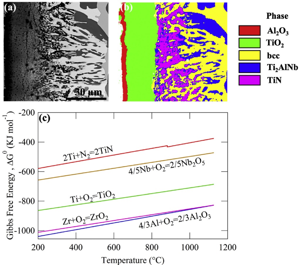
Fig. 9. (a) Cross-sectional microstructure and (b) corresponding EBSD phase map of \text{Al}_{0.75} after 100 h of exposure at 1,100 ^\circ\text{C} , and (c) plot of standard Gibbs free energy of formation for relevant oxides and nitrides.
