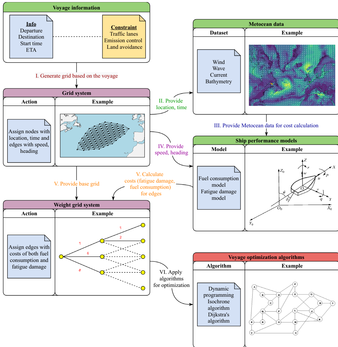
Fig. 9 A typical workflow of the voyage optimization process concerning various objectives, such as minimum fuel consumption, lowest fatigue damage and ETA, etc
