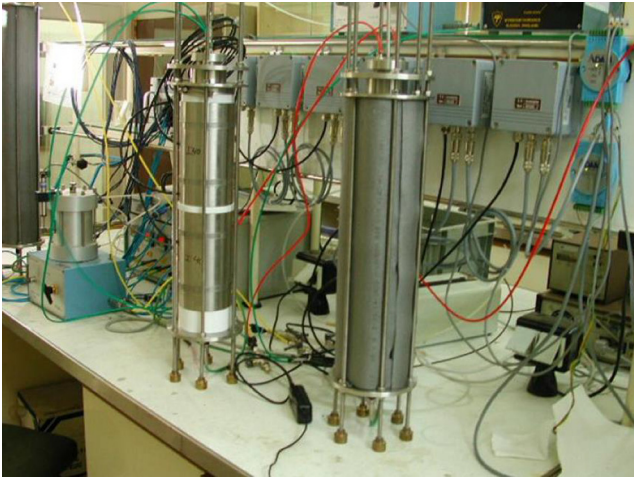
Fig. 8. CIEMAT infiltration cells [73].
