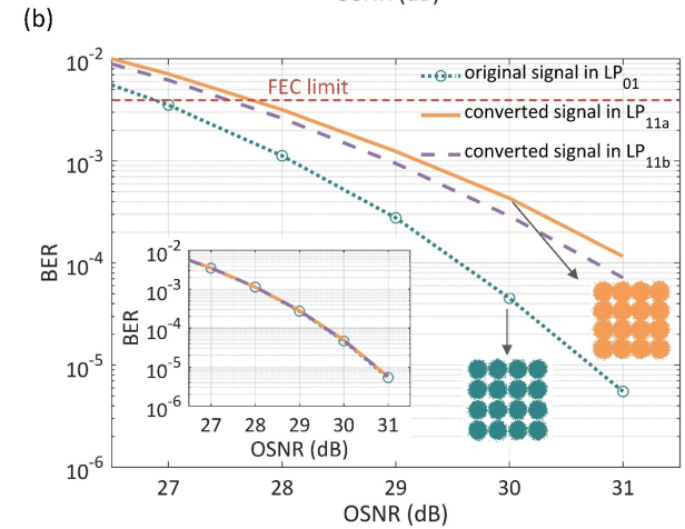
Fig. 12. BER of 100 Gbaud 16-QAM signal before and after mode-selective conversion, when signal wavelength is (a) 1557 nm and (b) 1565 nm. Inset of each subfigure shows the case when using 25 Gbaud 16-QAM signal.
