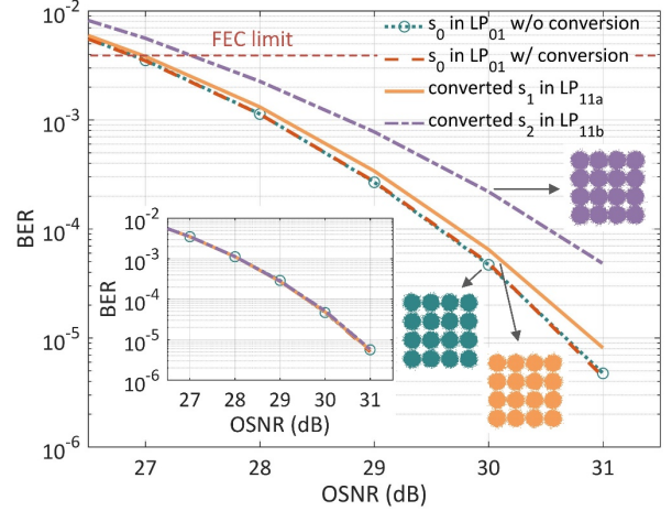
Fig. 14. BERs and constellations of 3 \times 100 Gbaud 16-QAM signals before and after three-wavelength to three-mode superchannel conversion. Inset shows the case when 3 \times 25 Gbaud 16-QAM signals are used.
