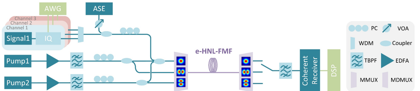
Fig. 7. System setup of the OXC based on the designed e-HNL-FMF. Abbreviations not included in main text: PC: Polarization controller; VOA: Variable optical attenuator; WDM: Wavelength-division multiplexer; DSP: Digital signal processing.
