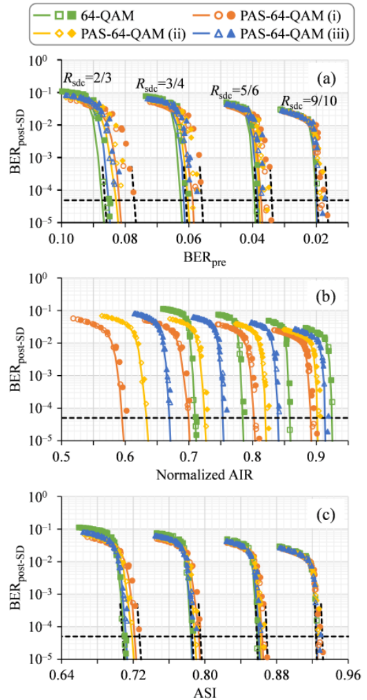
Fig. 8. Post-SD-FEC BER as a function of (a) pre-FEC BER, (b) normalized AIR, or (c) ASI on fiber-optic channel with bit mapping \mathbb{M}_{\text{FU}} .
