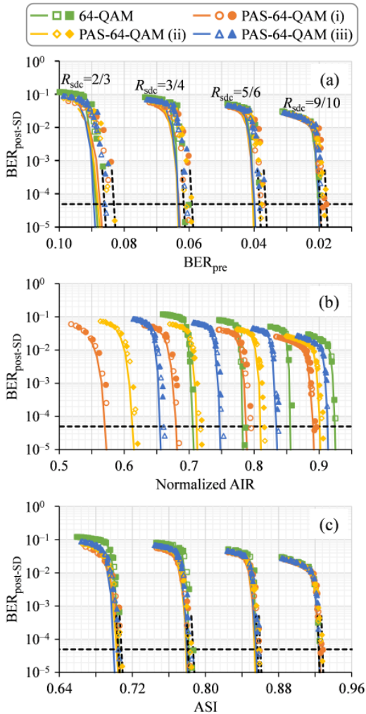
Fig. 7. Post-SD-FEC BER as a function of (a) pre-FEC BER, (b) normalized AIR, or (c) ASI on fiber-optic channel with bit mapping \mathbb{M}_{\text{FS1}} .
