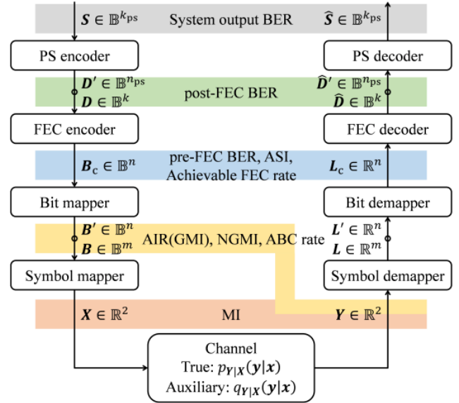
Fig. 1. System model of BICM with PS. Here we show the notations of the signals with the number of the dimensions and key performance metrics that will be discussed in this paper.
