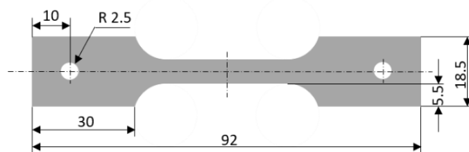
Figure 10. Sample geometry used for hot ductility tests; sample thickness: 3.5 mm.
