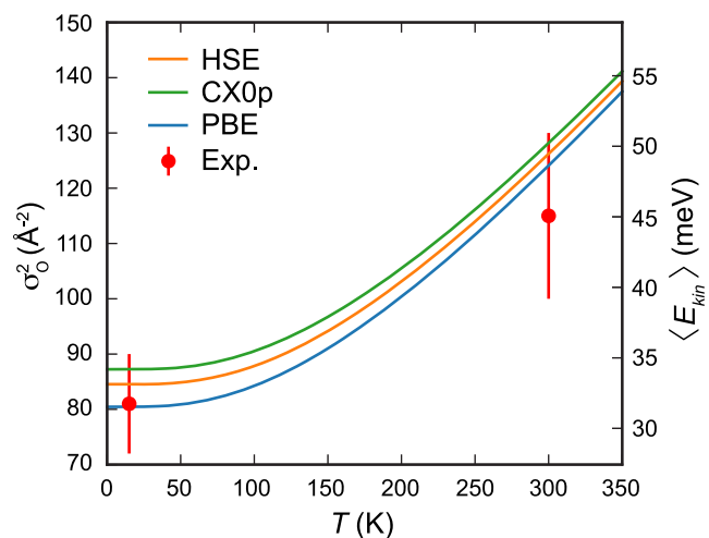
Figure 11. Calculated mean squared momentum averaged over the three directions \alpha ( \sigma_0^2 ) (left) and mean kinetic energy \langle E_{kin} \rangle (right) as a function of temperature. The bullets represent the experimental values of \langle E_{kin} \rangle .
