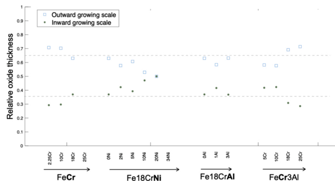
Fig. 8. Summary of the relative amounts of inward- and outward-growing scales for all model alloys in the secondary corrosion regime (exposed for 48 h in 5% O 2 + N 2 + 1 mg K 2 CO 3 (s) at 600°).
