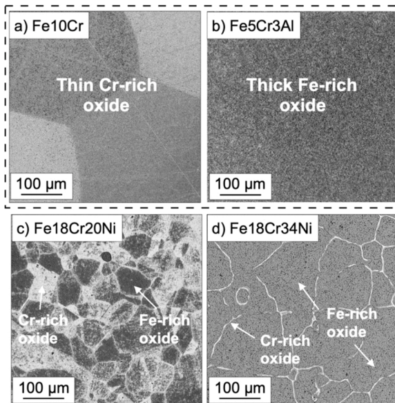
Fig. 4. Plan view BSE-SEM images of the type of oxide scales that formed after 24 h exposure in 5% O 2 + 95% N 2 at 600 °C. The thin Cr/Al-rich scale (a) was observed on the majority of the exposed model alloys, while the Fe-rich oxide (b) was observed on parts of the surfaces of the alloys with low Cr content (Fe 2.25 Cr [20], Fe 5 Cr 3 Al) and on several alloy grains on the Fe 18 Cr 20 Ni (c). The Fe 18 Cr 34 Ni alloy (d) formed Fe-rich oxide on the alloy grains and a thinner Cr-rich oxide on top of the alloy grain boundaries.
