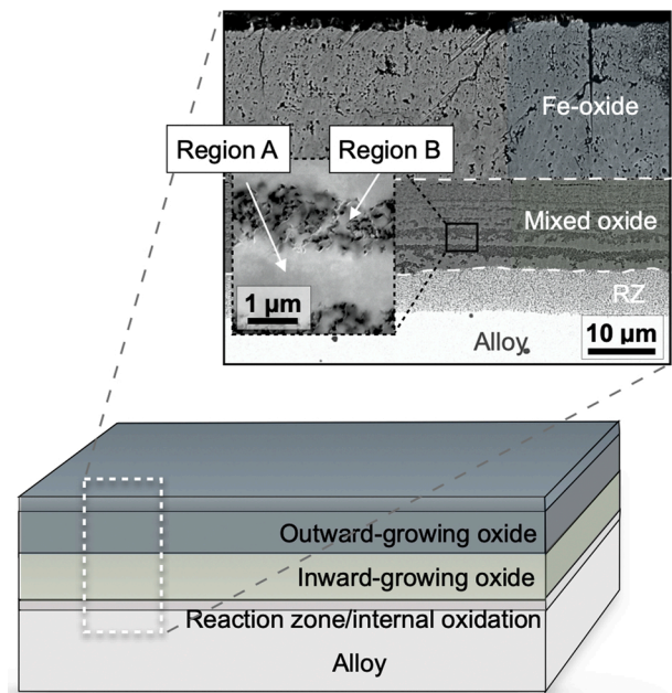
Fig. 5. Example of the oxide scale formed in the secondary regime on Fe-based alloys at 600 °C. The oxide scale is composed of outward-growing iron oxide (Fe 2 O 3 /Fe 3 O 4 ) and an inward-growing mixed (Fe, Cr, Al/Ni) oxide. The inward-growing oxide typically has a banded microstructure with alternating bright (region A) and dark (region B) contrast and a reaction zone type of internal oxidation at the scale/metal interface.
