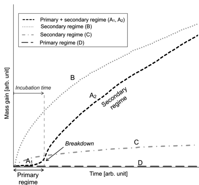
Fig. 1. Kinetic illustration of the primary (A 1 , D) and secondary (A 2 , B, C) corrosion protection of Fe-based alloys. The primary (A 1 ) and secondary (A 2 ) regimes are marked in the figure along with the breakaway event and incubation time. Note that the breakaway event occurs instantly in curve B and C.
