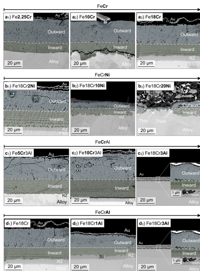
Fig. 6. BSE-SEM images of the oxide scales formed after 48 h exposure in 5% O_2 + N_2 + 1 \text{ mg } K_2CO_3(s) at 600^\circ C on (a) FeCr, (b) FeCrNi, (c,d) FeCrAl alloys. The different types of layers are falsely colored (post-processed) to simplify for comparisons between the oxide layers formed on different alloys. A region of internal oxidation is indicated by the majority of the samples, where the most common type is the reaction zone (RZ).
