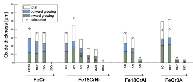
Fig. 7. Summary of the measured oxide scale thicknesses for all model alloys exposed for 48 h in 5% O 2 + 95% N 2 + 1 mg K 2 CO 3 (s) at 600 °, including the estimated thicknesses calculated from mass gain data (◇). Note that the oxide scale formed on the Fe18Cr34Ni alloy was not examined in cross section.
