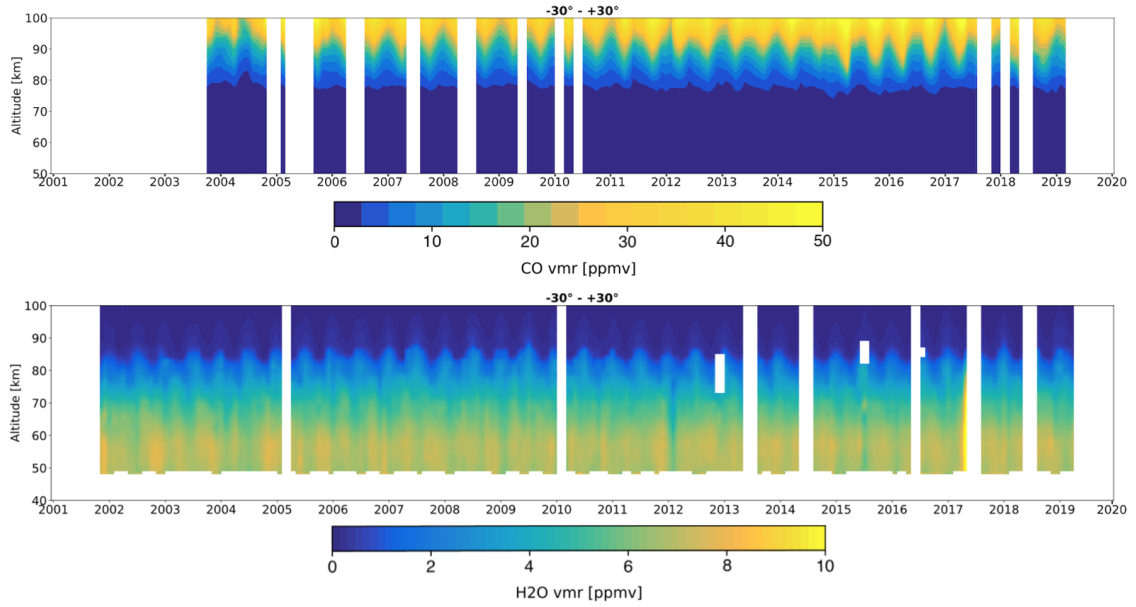
Figure 2.3: Time series of CO (top) and H 2 O (bottom) volume mixing ratios measured by SMR for the -30^{\circ} - +30^{\circ} latitude band, taken from Paper 1 and 2 respectively. The white bands indicate periods during which the number of scans in the given latitude band is lower than 10. The ticks on the x-axis correspond to the beginning of each year. Note the two different colour scales.
