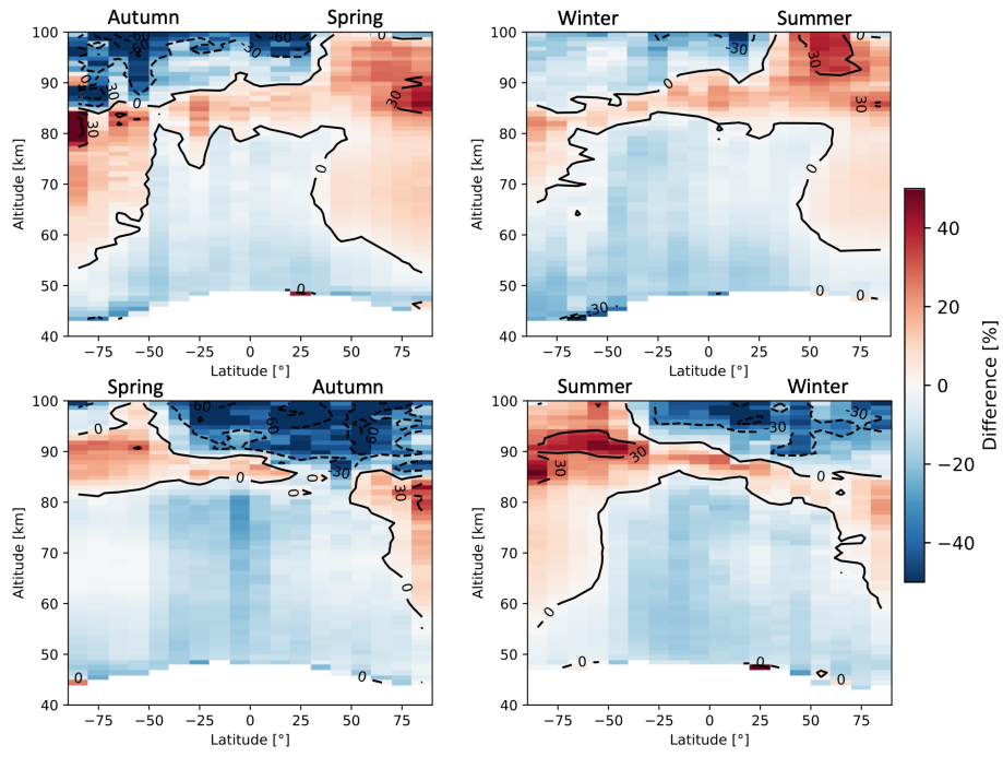
Figure A1. Seasonal zonal means of H 2 O FM13 SMR v3.0–v2.1 relative differences averaged over the whole time period between February 2001 and April 2019. The seasons are intended as the time between solstice and equinox.
