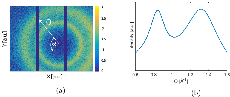
Figure 3.4: Experimental SAXS data of P14TFSI in (a) two dimensions and (b) one dimension.
