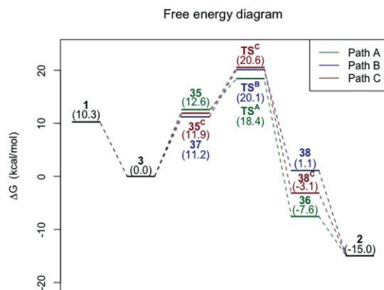
Figure 3. Computed free energy (298.15 K, 1 M) diagram for path A–C. A superscript C ( X^C ) denotes the corresponding structures without coordination of DBUH + . Energies relative to the 1,3-diketone 3 and free MeOH are shown in kcal/mol.
