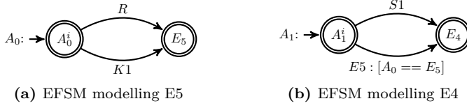
Figure 3: EFSMs for intermediate failure events, E4 and E5 of the fault tree
