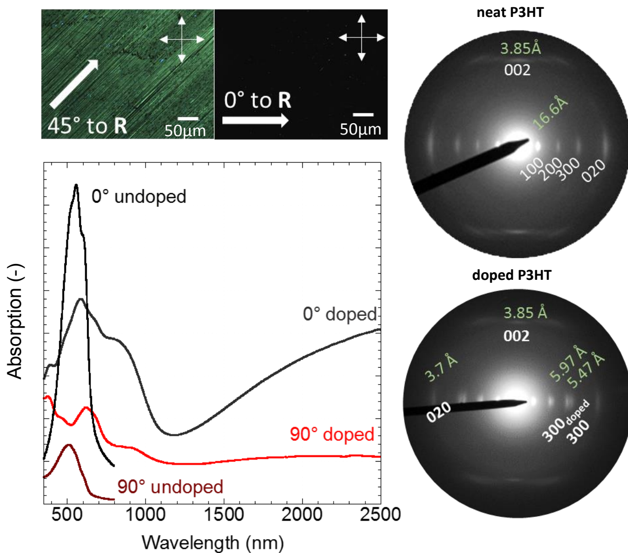
Figure 3.1. Top left: Polarised light optical microscopy images of rubbed P3HT films doped by \text{Mo}(\text{tfd-COCF}_3)_3 . Polariser and analyser orientations are shown to be crossed. Bottom left: Representative UV-Vis absorption spectra of oriented P3HT films in their undoped and doped states in parallel ( 0^\circ ) and in perpendicular ( 90^\circ ) to the rubbing direction. Data is shifted in y-direction for clarity. Right: ED patterns of rubbed P3HT films before (top) and after doping (bottom) by \text{Mo}(\text{tfd-COCF}_3)_3 .
