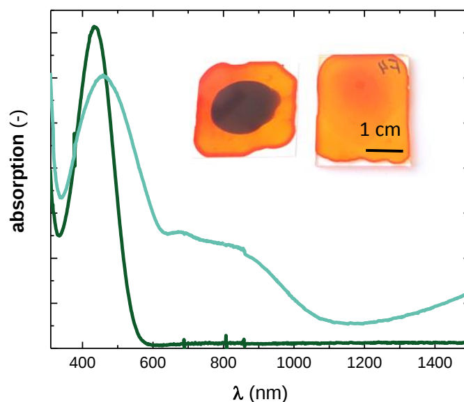
Figure 2.2. Representative UV-vis spectra of drop cast regiorandom (regioregularity 28%) P3HT (dark green) doped with Mo(tfd-COCF 3 ) 3 (light green); measured conductivity of 0.09 S cm -1 , inset pictures of regiorandom P3HT doped with Mo(tfd-COCF 3 ) 3 (left) and F4TCNQ (right).
