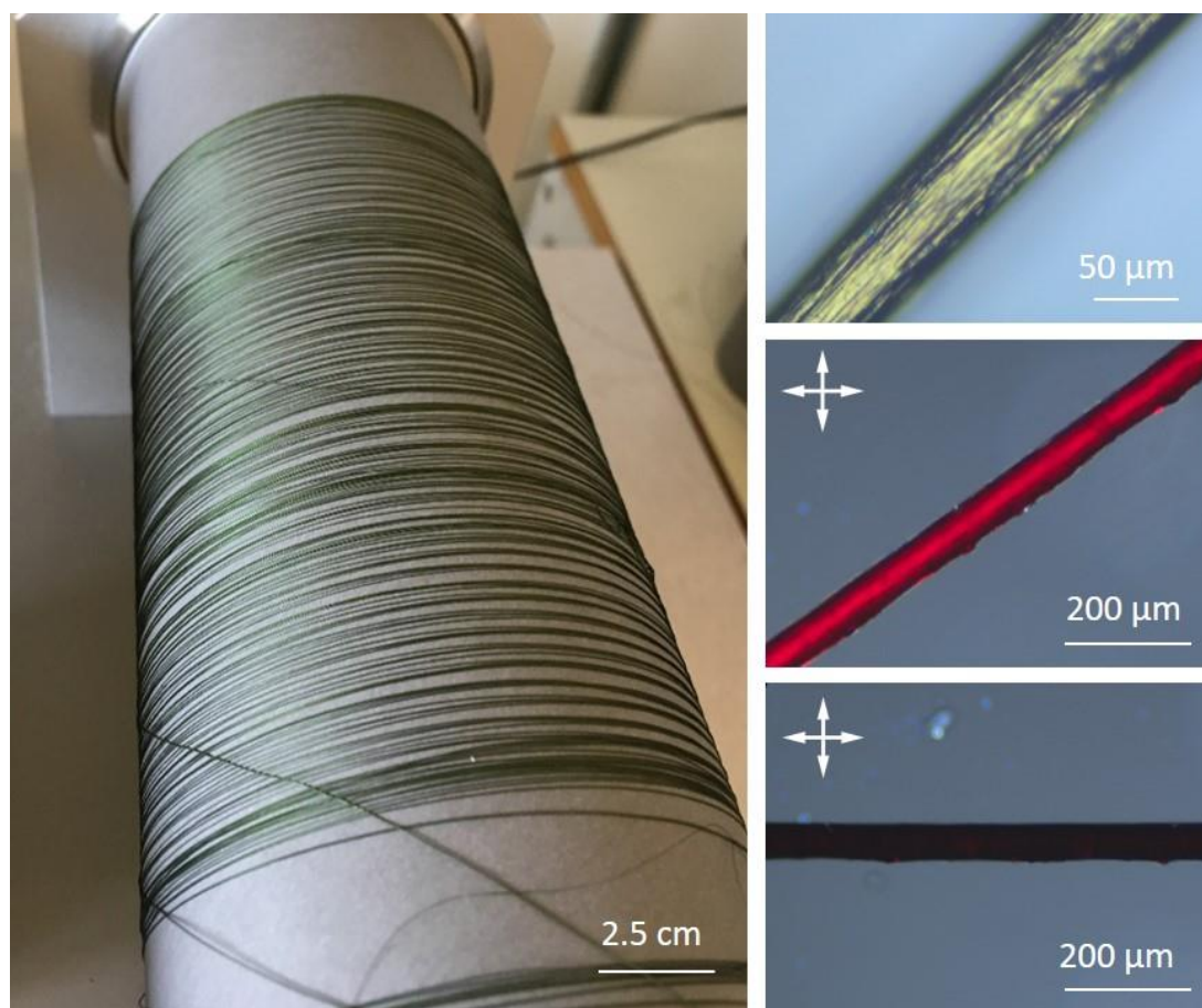
Figure 5.4. Left: Photograph of melt spun fibre Right: Optical light microscope (reflective light) image of the fibre surface (top), polarised light microscopy image of a melt spun fibre 45° (middle) and 0° (bottom), fibre spinning direction is set parallel to the polarisation of the incident light.
