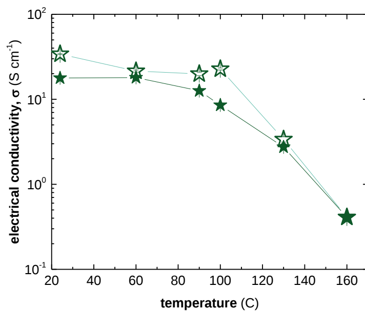
Figure 2.8. Electrical conductivity as a function of temperature for \text{Mo}(\text{tfd-COCF}_3)_3 doped thin films of P3HT, not-annealed film (open stars) pre-annealed films at 120°C for 30 min (closed stars).
