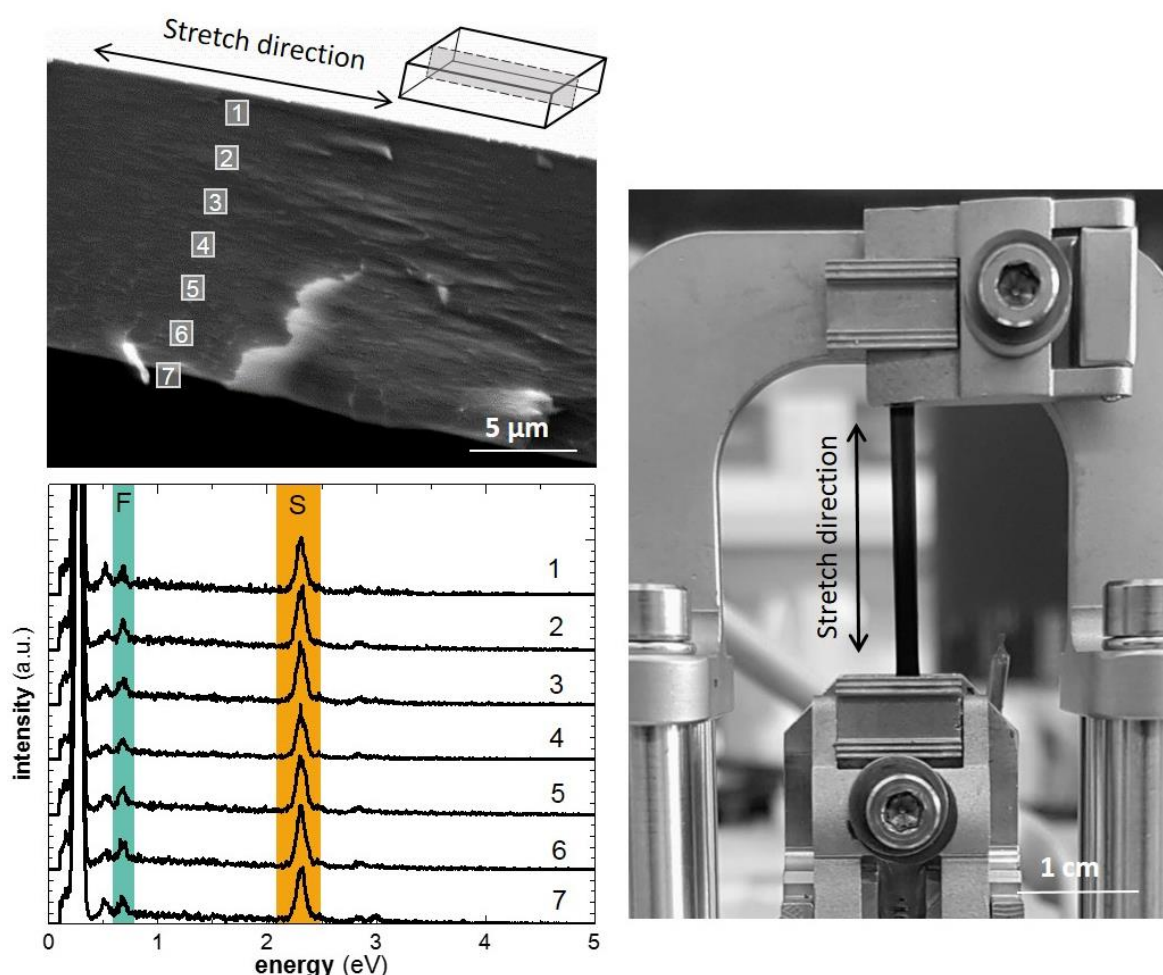
Figure 4.1. Top left: Scanning electron microscopy (SEM) image of the freeze-fractured surface used for EDX; inset: sketch of EDX sample, the freeze fractured surface is shown by the dashed line. Bottom left: EDX spectrogram of stretched P3HT sequentially doped with \text{Mo}(\text{tfd-COCF}_3)_3 for 72 h; fluorine and sulphur peaks are coloured green and orange respectively, the S/F ratio varied between 0.3 to 0.5 across the tape. Right: Stretched film of P3HT, clamped in a DMA instrument.
