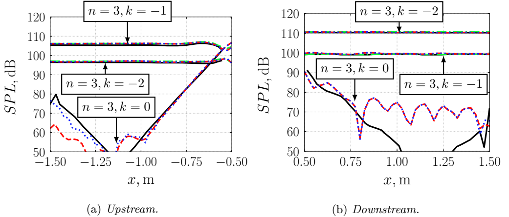
Figure B.11: Variation in amplitude of pressure modes spinning at three times the fundamental frequency (— HYDLIN [9], - - - Mu^2 s^2 T - L [19], - - - G3D::Flow (direct approach), ..... G3D::Flow (reformulation using characteristic variables)).
