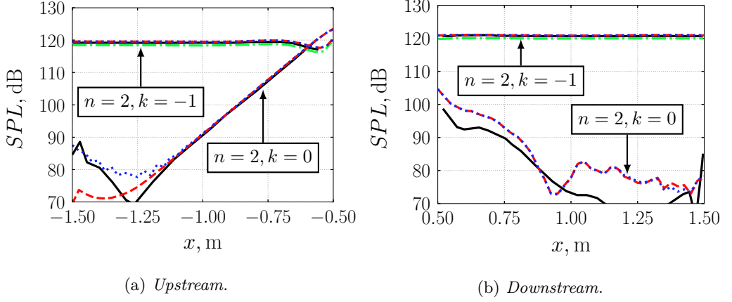
Figure B.10: Variation in amplitude of pressure modes spinning at twice the fundamental frequency (— HYDLIN [9], - - - Mu^2 s^2 T - L [19], - - - G3D::Flow (direct approach), ..... G3D::Flow (reformulation using characteristic variables)).
