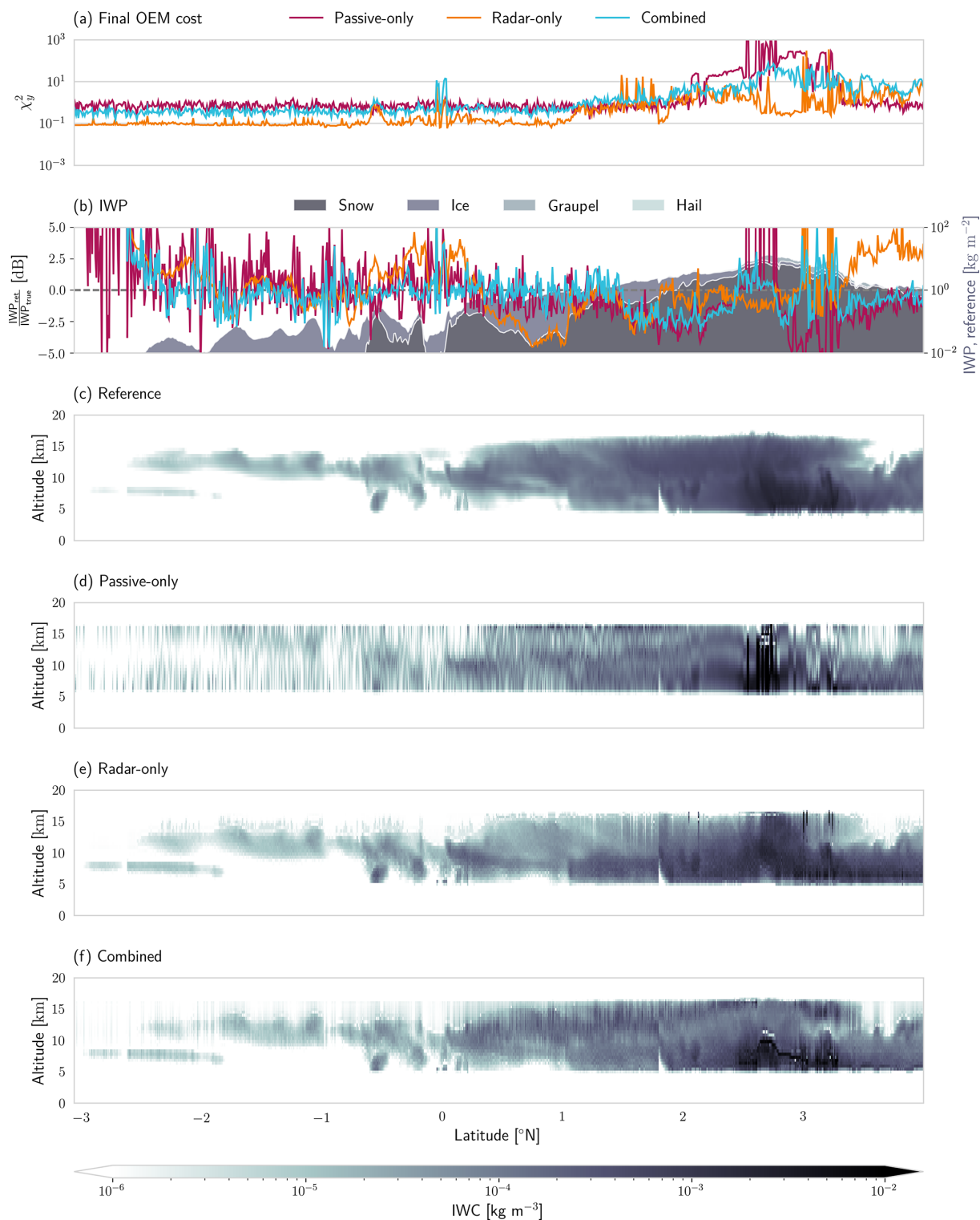
Figure 7. Results of the ice hydrometeor retrieval for the first test scene using the Large Plaque Aggregate particle model. Panel (a) displays the value of the \chi^2 diagnostic normalized by the dimension of the measurement space of the corresponding retrieval. Panel (b) displays retrieved IWP in decibels (dB) relative to the reference IWP. Reference IWP and the contributions from different hydrometeor classes are displayed by the filled areas in the background. Panel (c) shows the reference IWC from the model scene. Panels (d), (e) and (f) display the retrieval results for the passive-only, radar-only and combined retrieval, respectively.
