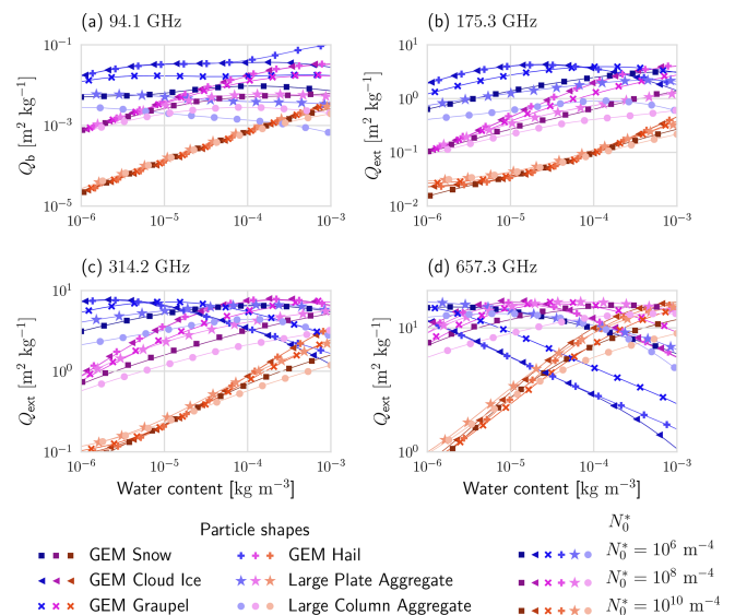
Figure 4. Bulk mass backscattering coefficient Q_b at (a) 94.1 GHz and mass attenuation coefficients Q_e at frequencies (b) 175.3 GHz, (c) 314.2 GHz and (d) 657.3 GHz for the particle models used in the simulated observations and the retrieval. Different colors show the bulk properties for different values of the N_0^* parameter of the PSD.
