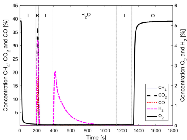
Fig. 13. One cycle of water splitting experiment split up to different phases. 5 g LD slag and 10 g sand were used as bed material and the temperature was set to 870 °C “I” = Inert flush. “R” = reduction with CO. “H 2 O” = Oxidation with steam resulting in water splitting and generation of H 2 . “O” = Oxidation with 5% O 2 .
