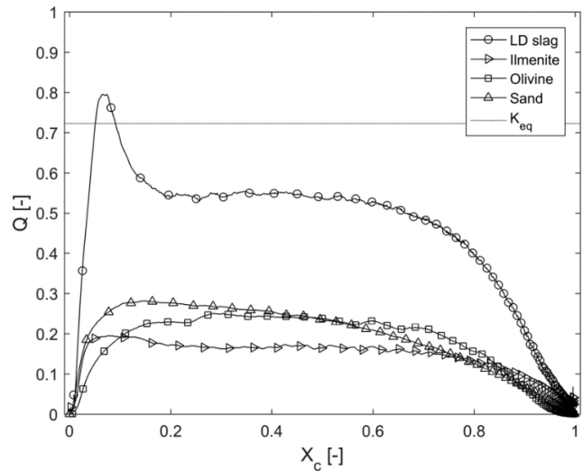
Fig. 10. The reaction quotient ( Q_i ) related to the WGS reaction for LD slag, ilmenite, olivine and silica sand plotted against the char conversion fraction X_c for one cycle at 870 °C. The plotted cycle is the same as in Fig. 5. The equilibrium constant ( K_{eq} ) at 870 °C for the WGS reaction is given as a dotted line. Since no H_2O is measured in the outgoing gas the H_2O concentration was assumed to be 50%, same as in the incoming gases to the reactor.
