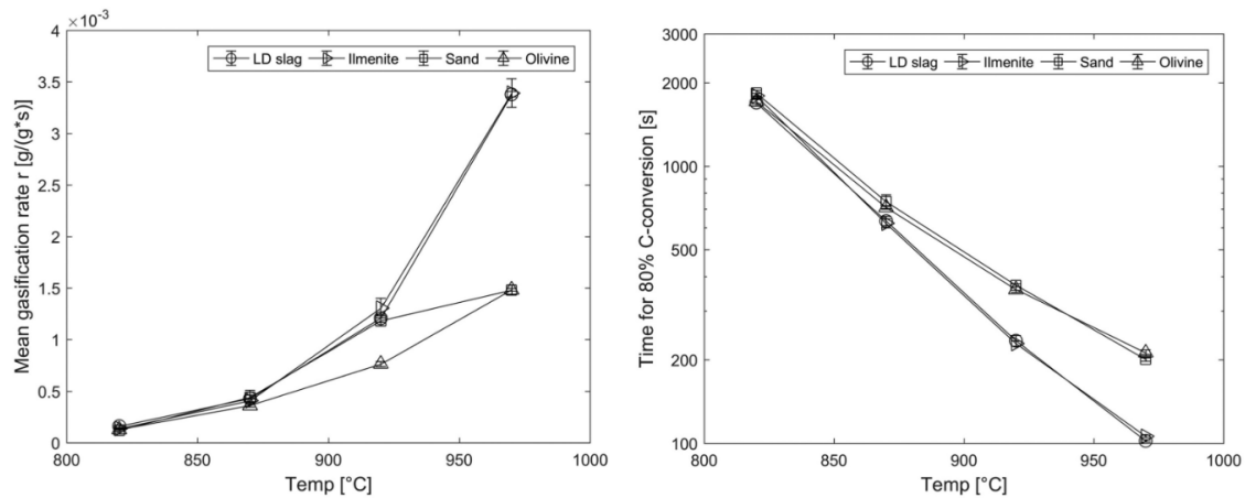
Fig. 6. Left: mean gasification rate ( r ) for 0.3 < X_c < 0.7 of the biochar for the investigated bed materials different temperatures using 0.2\text{ g} fuel. Right: Time required to convert 80\% of the carbon in the biochar to CO , CO_2 and CH_4 .
