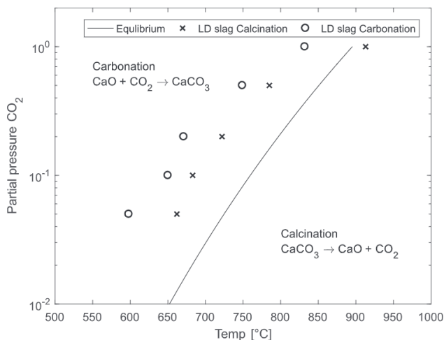
Fig. 16. Equilibrium curve and experimental results of temperature where carbonated LD slag calcine (x) and are carbonated (o) at a different partial pressure of \text{CO}_2 . The equilibrium curve is for reaction (R7) and is dependent on both partial pressure \text{CO}_2 and temperature.
