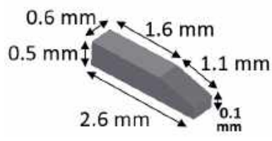
Figure 5.27: Dimensions of the machined HR Si taper (Paper D)
