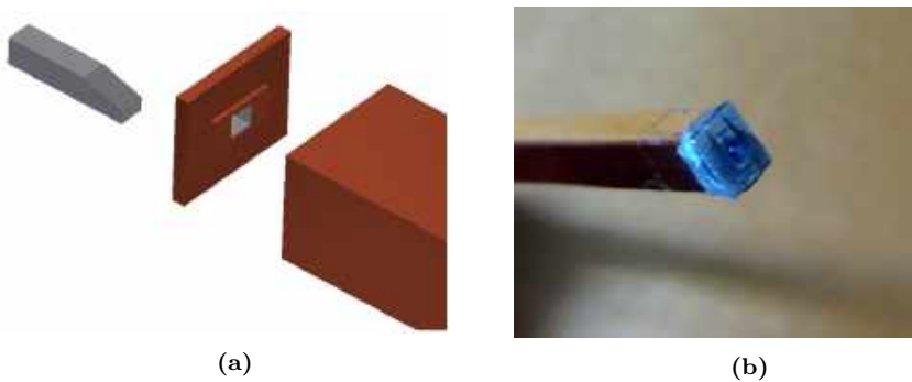
Figure 5.29: Assembly of the interconnect using metal holder (a) Illustrative view (b) Photo of the realized interconnect
