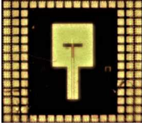
Figure 5.30: Photo of the fabricated eWLB (Paper D)
