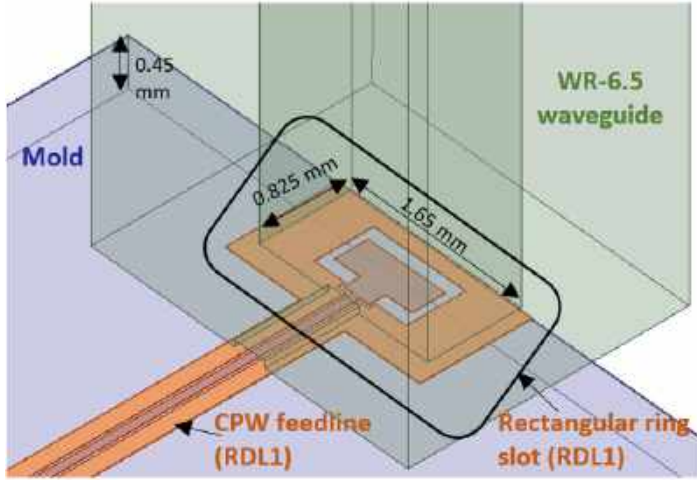
Figure 5.18: Illustration of the rectangular slot ring transition (Paper C)
