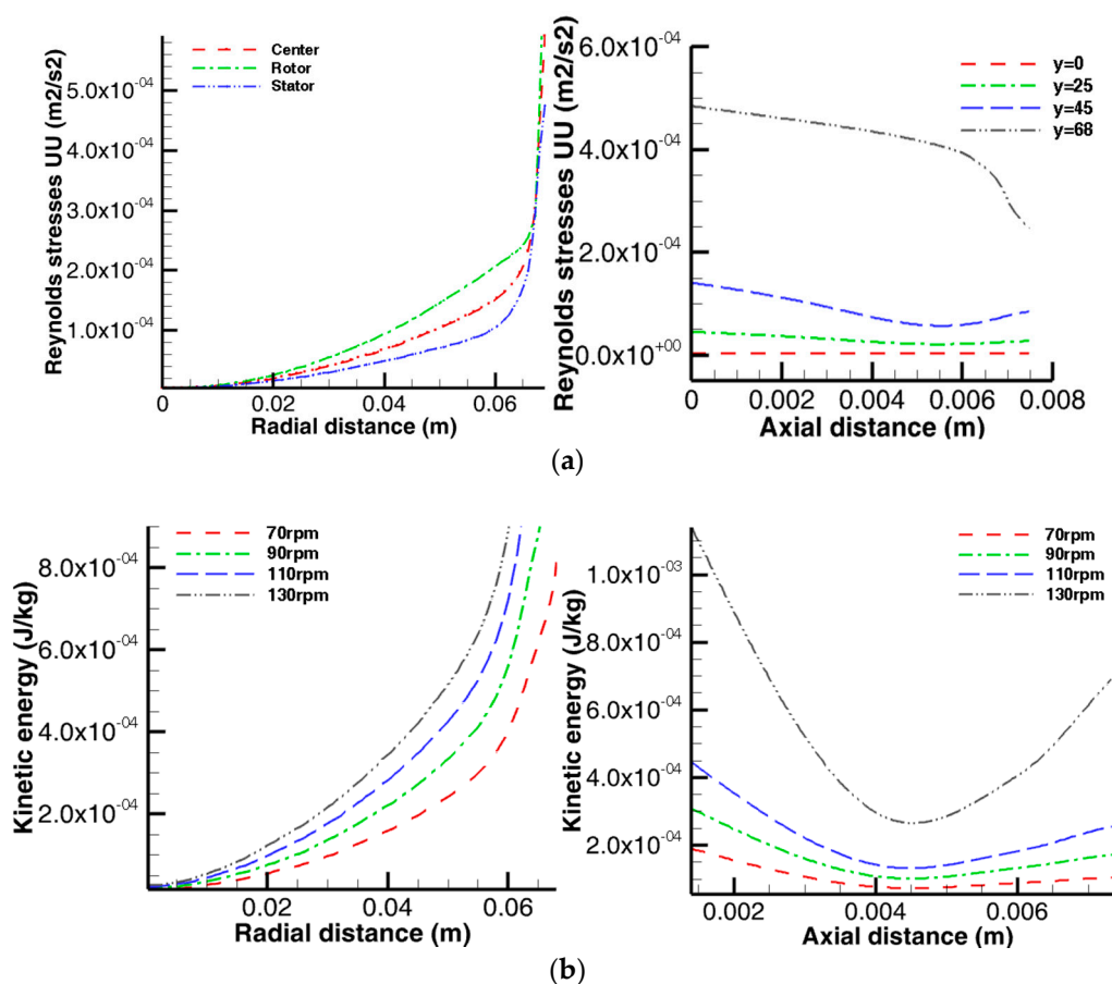
Figure 9. Spatial distribution of the turbulence and mixing intensities (a) Reynolds stress distributions on the Y-Z plane at x = 0.0015, 0.003725, \text{ and } 0.006 , and X-Z plane parallel to the shaft at y = 0, 0.025, 0.045, \text{ and } 0.068 . (b) Turbulent kinetic energy distribution on the Y-Z plane at x = 0.003725 and X-Z plane parallel to the shaft at y = 0.025 for N = 70\text{--}130 rpm.
