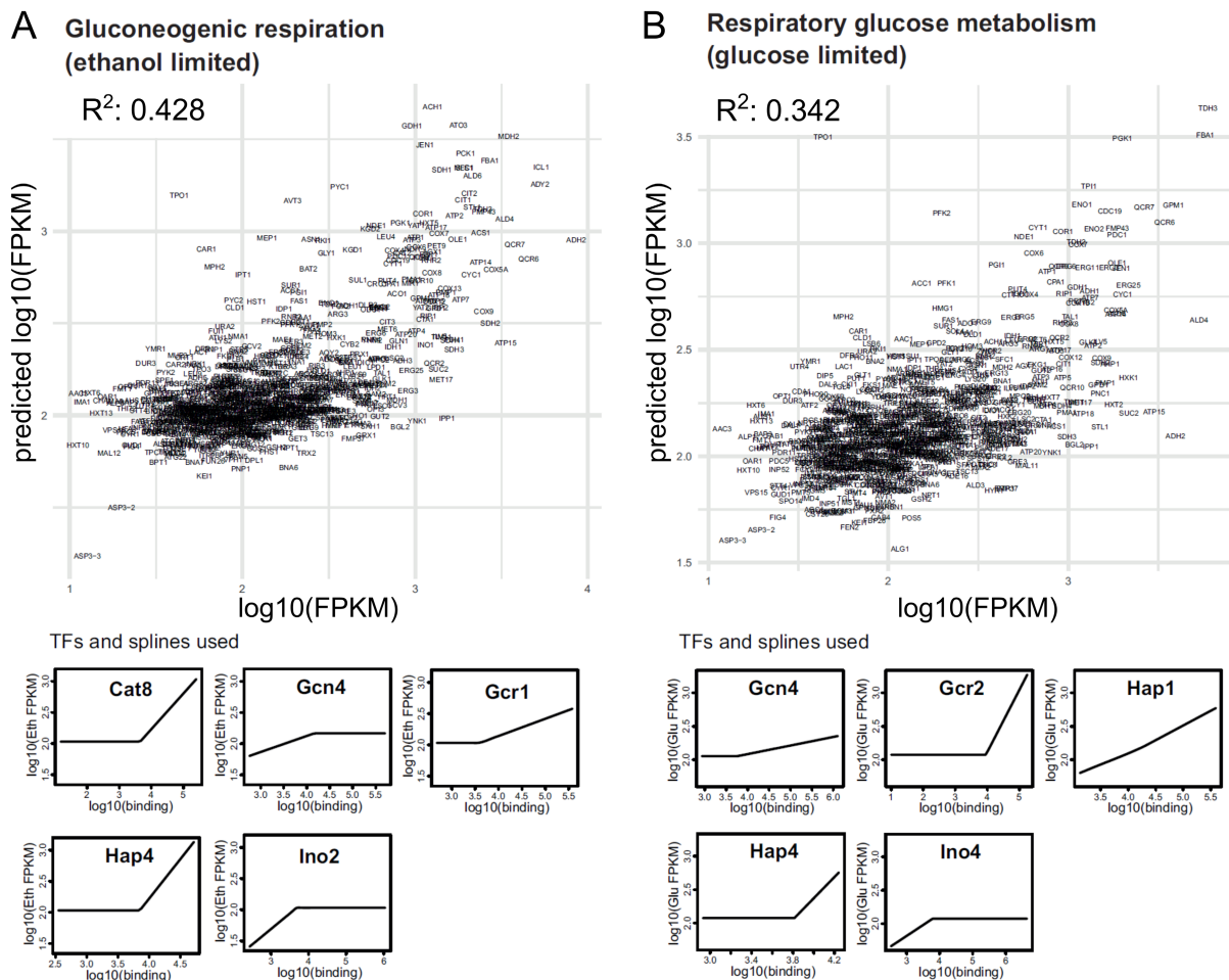
Figure 17: Results for multivariate adaptive regression splines models used to predict gene transcript levels. A: Cross-validated predictions for gene expression levels in ethanol-limited condition. Selected TFs and splines are shown below. B: Cross-validated predictions for gene expression levels in glucose-limited condition. Selected TFs and splines are shown below. FPKM: fragments per kilobase per million reads mapped.
