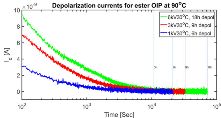
Figure 3-15. The minimum depolarisation time required at 90°C
