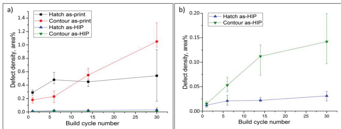
Figure 31. Defect density in samples built from progressively re-used powder; (a) as-printed and as-HIP condition; (b) as-HIP condition [81].
