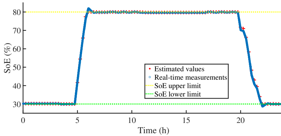
Figure 6.24: The estimated SoE of the BES dispatch model during the demonstration of Model-1 at HSB LL building and the real-time value of SoC as measured by the converter (updated per 5 seconds).
