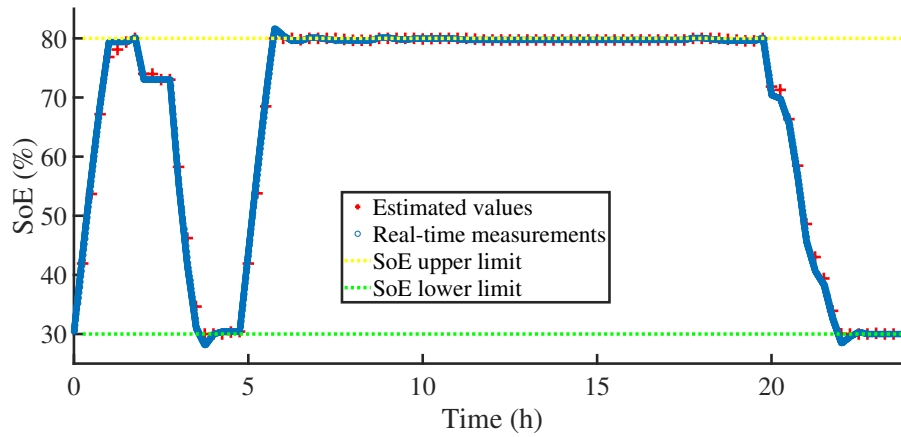
Figure 6.25: The estimated SoE of the BES dispatch model during the demonstration of Model-2 at HSB LL building and the real-time value of SoC as measured by the converter (updated per 5 seconds).
