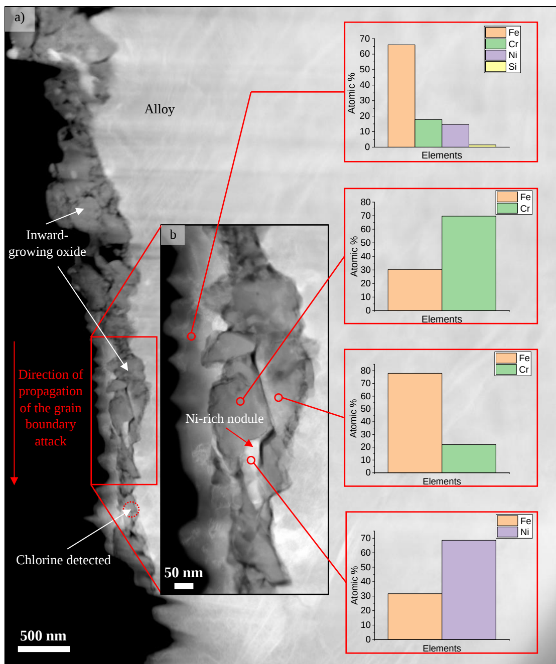
Figure 45: Micrograph showing the HAADF image of thin foil (a) lower, and b) higher magnification image of a grain boundary attack from a 304L sample exposed to 5% O 2 + 20%H 2 O + N 2 (bal.) for 24 hours at 600 °C under continuous KCl deposition (red box labelled "TEM lamella 2" in Figure 42c). Locations of quantitative analyses and their corresponding results are represented in at.%.
