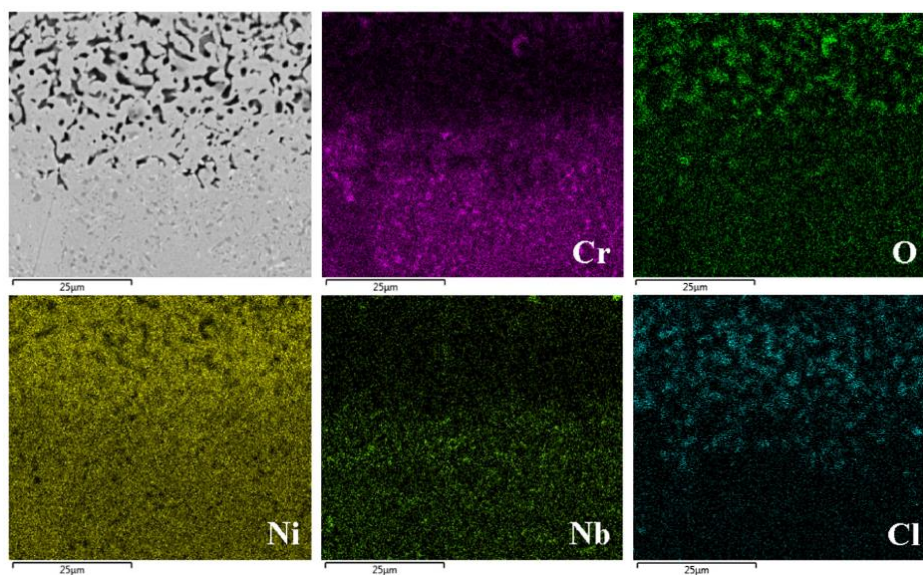
Figure 48: SEM image using BSE and EDX maps at the corrosion front of the aged Ni35Cr4Nb alloy exposed with pre-deposited KCl for 168 hours at 600 °C in 5% (vol/vol) \text{O}_2 (g) + 15% (vol/vol) \text{H}_2\text{O} + \text{N}_2 (g; balance) atmosphere [100].
