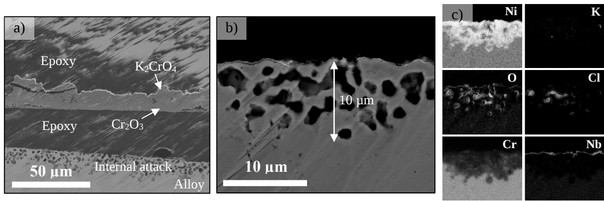
Figure 49: a) and b) BSE images of the solution-treated Ni35Cr4Nb exposed for 24 hours under continuous KCl deposition in 5% (vol/vol) O_2 (g) + 15% (vol/vol) H_2O + N_2 (g; balance) atmosphere. c) EDX maps of b) [100].
