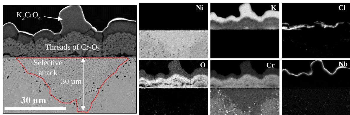
Figure 50: SEM image using BSE and EDX maps of the aged Ni35Cr4Nb exposed for 24 hours under continuous KCl deposition in 5% (vol/vol) O_2 (g) + 15% (vol/vol) H_2O + N_2 (g; balance) atmosphere. The Nb signal could be a false signal that overlaps with sputtered gold.
