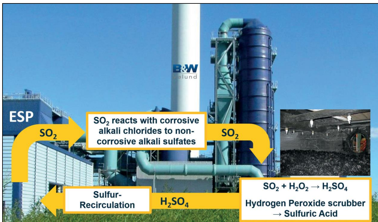
Figure 29: The flue gas treatment of MEC consists of an ESP (Electrostatic Precipitator), an HCl scrubber, a multistage scrubber for \text{SO}_2 removal, dioxin removal using ADIOX[115], and flue gas condensation[109].
