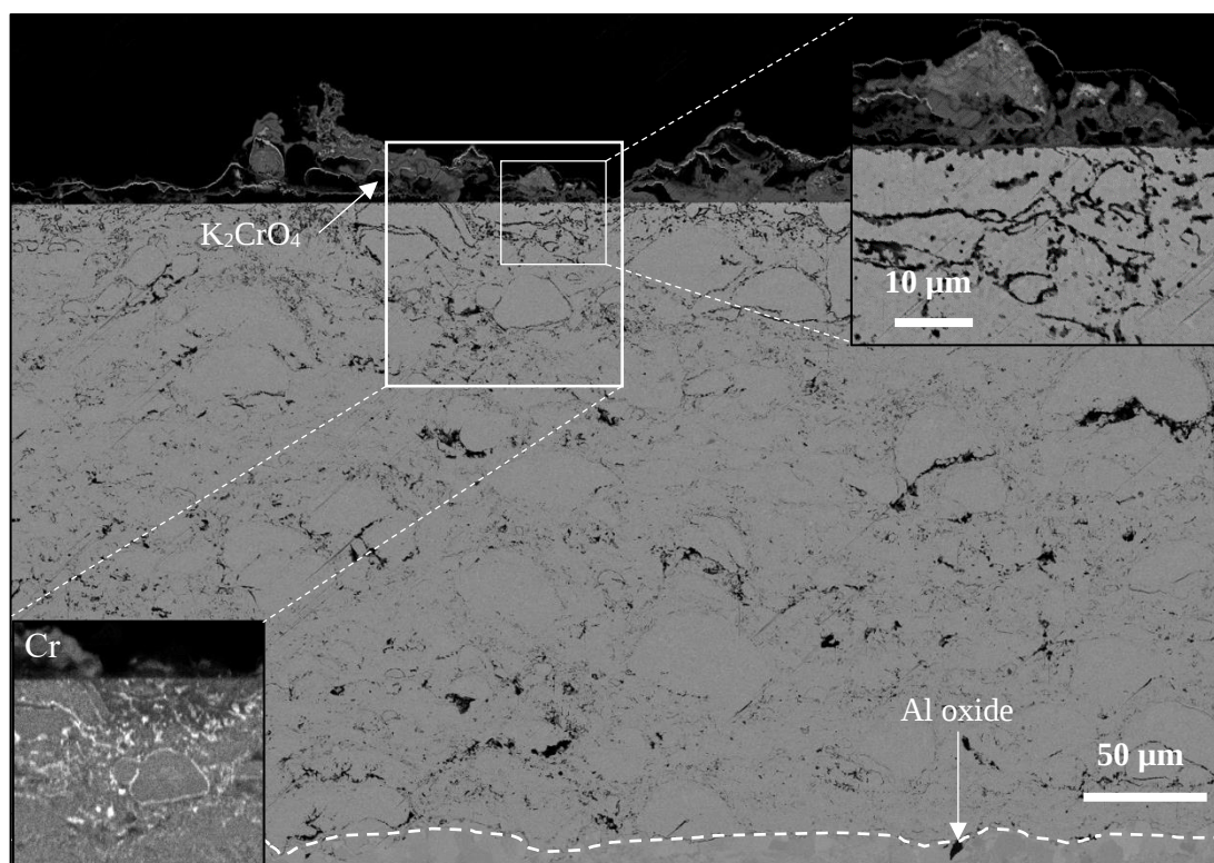
Figure 60: SEM image using BSE of a cross-section of a NiCrAlY-coated sample after exposure to 5% O_2 + 20% H_2O + N_2 + 1.0 mg/cm^2 at 600 °C for 168 hours. The signal for chromium from the EDX analysis is located at the bottom left of the picture. A higher magnification of the surface is shown at the top right. The dashed line represents the coating/substrate interface.
