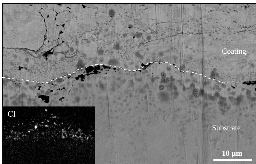
Figure 58: SEM image using BSE of a cross-section of the coating/substrate interface of a NiCr-coated sample after exposure to 5% O 2 + 20% H 2 O + N 2 + 1.0 mg/cm 2 at 600 °C for 168 hours. The signal for chlorine from the EDX analysis is located at the bottom left of the picture. The dashed line represents the coating/substrate interface.
