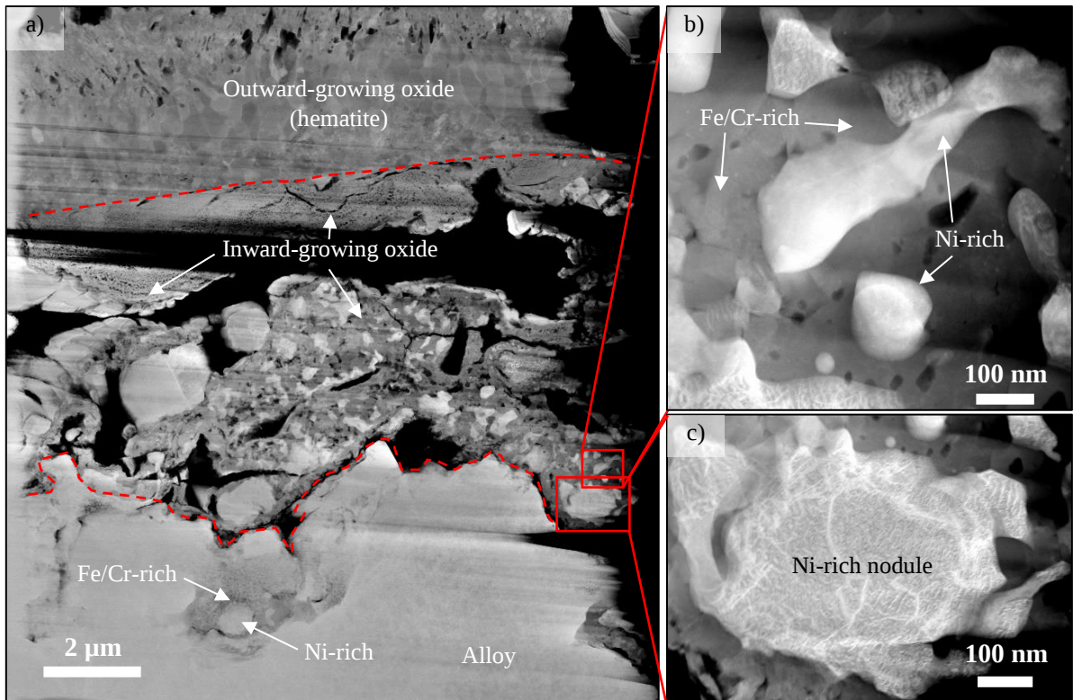
Figure 43: a) Micrograph showing the HAADF image of a thin FIB lamella of 304L sample exposed to 5% O 2 + 20% H 2 O + N 2 (bal.) at 600 °C for 24 hours under continuous KCl deposition (red box labelled "TEM lamella 1" in Figure 42c; b) high magnification image of the typical inward-growing oxide region showing Cr-rich (in grey) and Ni-rich nodules (in bright), and c) high magnification of a Ni-rich nodule.
