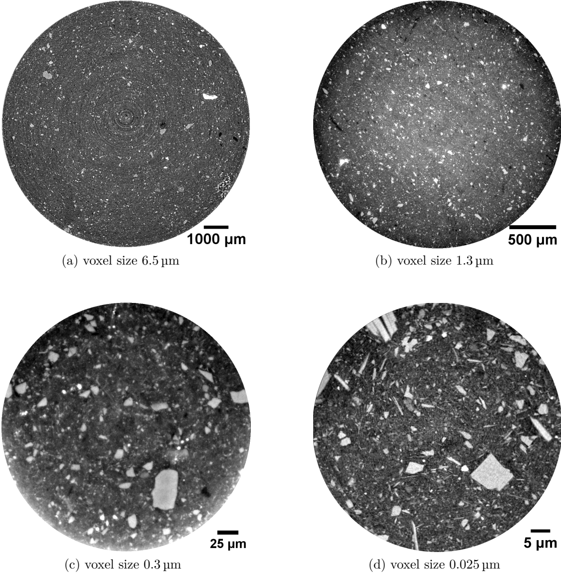
Figure 3.12: Phase contrast tomographies of sensitive clay samples from Utby at different magnification levels.
