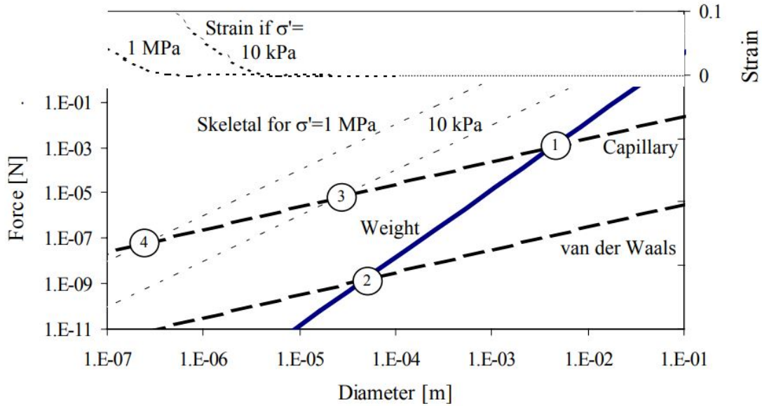
Figure 2.12: Different type of forces (skeletal, capillary, electrical) on soil particles. The upper part of the figure shows the strain (axis on right) caused by changing the pore fluid ionic concentration from fresh-water to seawater conditions (Santamarina, 2003).
