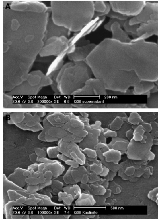
Figure 2.6: SEM micrographs of kaolinite at high magnification (A) and low magnification (B) (Du et al., 2009).
