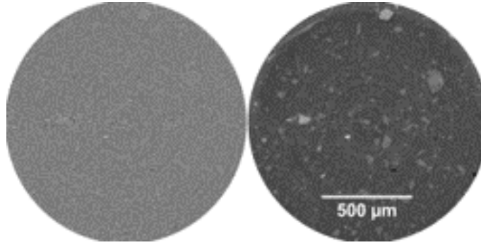
Figure 3.10: Tomographic sections of sensitive clay specimens (Utby clay), using absorption (left) and phase (right) contrast techniques.
