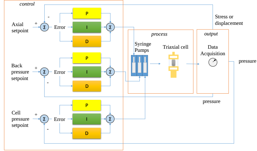
Figure 3.15: Flow chart of the control system for the miniature triaxial apparatus.
