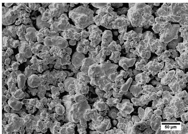
Fig. 1. Overview of as-received water-atomized iron powder.
