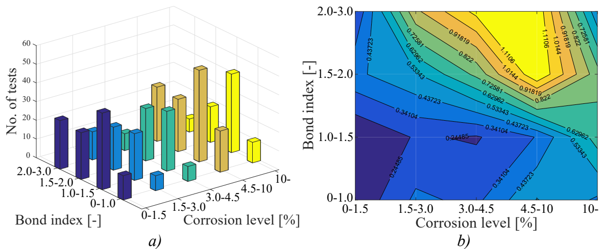
Figure 5.4. a) Four bond index (confinement) intervals and five corrosion level intervals on the horizontal axes and number of test results in each group on the vertical axes and b) contour plot of the coefficient of variation for relative bond strength in the database for varying bond index and corrosion level. Adopted from Paper II .
