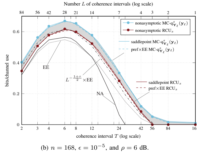
Fig. 2. R^*(L, T, \epsilon, \rho) as a function of L for a fixed n = LT .
