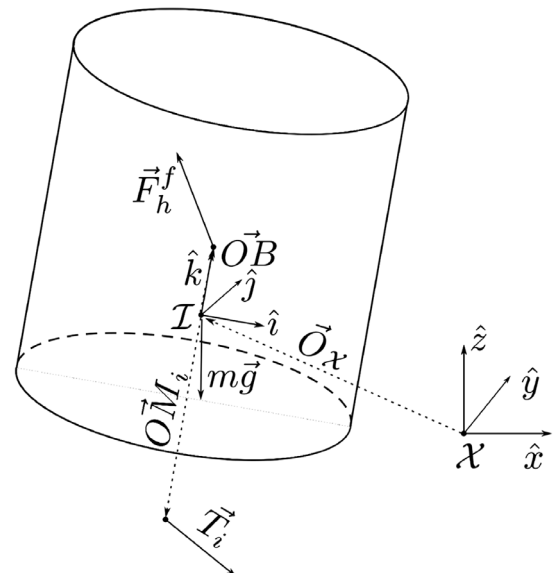
Fig. 2. Schematic view of the relation between the body-fixed coordinate system I and the inertial frame \mathcal{X} .
