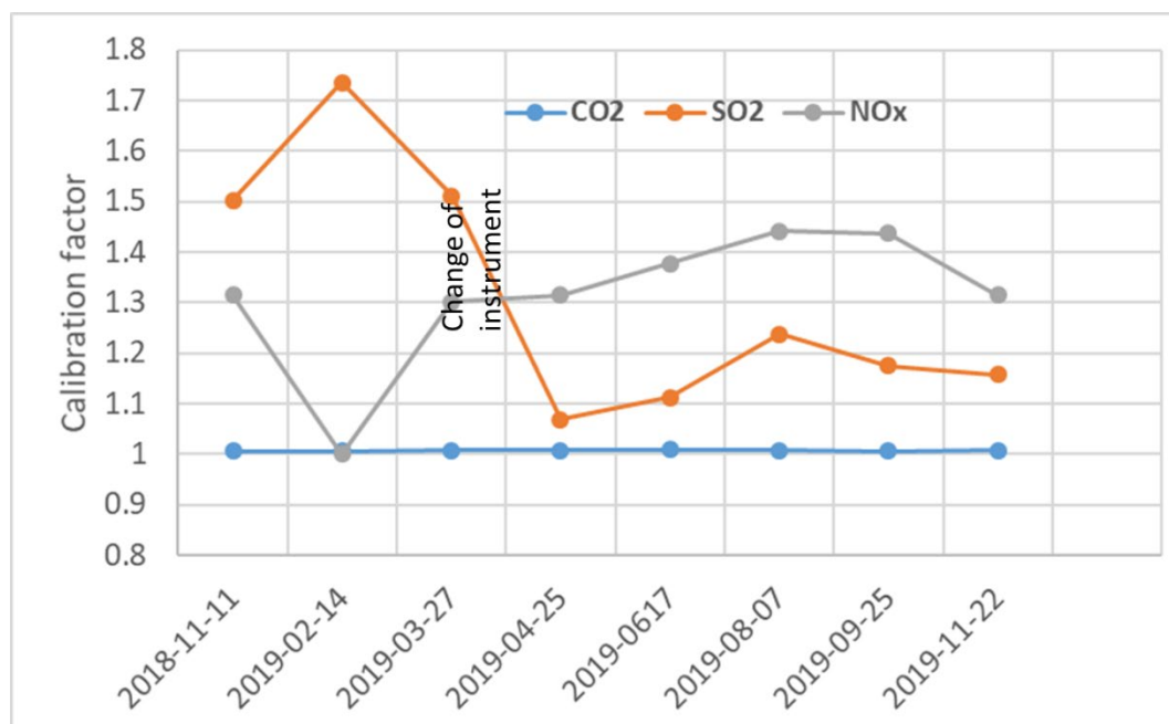
FIGURE 6. The calibration factors obtained during 2019 through measurements of gas standards from Air liquide.
