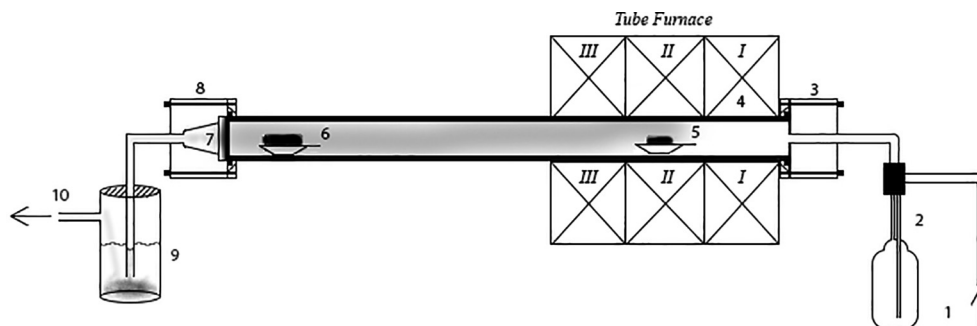
Fig. 1. The experimental schematics: (1) gas inlet, (2) atomizer, (3) inlet, (4) Al 2 O 3 -tube, (5) the precursor location, (6) the metallic coupon, (7) filter, (8) connector, (9) a sodium hydroxide solution (0.1 M) trap, and a water trap, and (10) the gas outlet.
