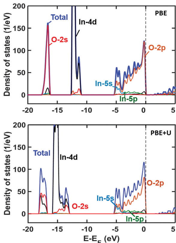
Fig. 1 Density of states for bulk In 2 O 3 using PBE and PBE+ U .
