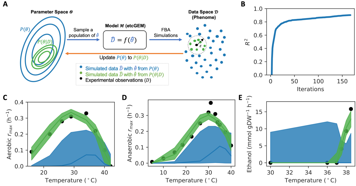
Figure 12 Uncertainty reduction and quantification with Bayesian statistical learning approach. (A) Overview of Bayesian genome scale metabolic modelling. (B) Minimal coefficient of determination score ( R^2 ) of Posterior models during SMC-ABC approach. (CD) Simulated (C) aerobic and (D) anaerobic growth rates in batch cultivations at various temperatures with Prior and Posterior etcGEMs. (E) Simulated ethanol secretion flux in chemostat at various temperatures. In (CDE), lines indicate median values and shaded areas indicate regions between the 5-th and 95-th percentiles.
