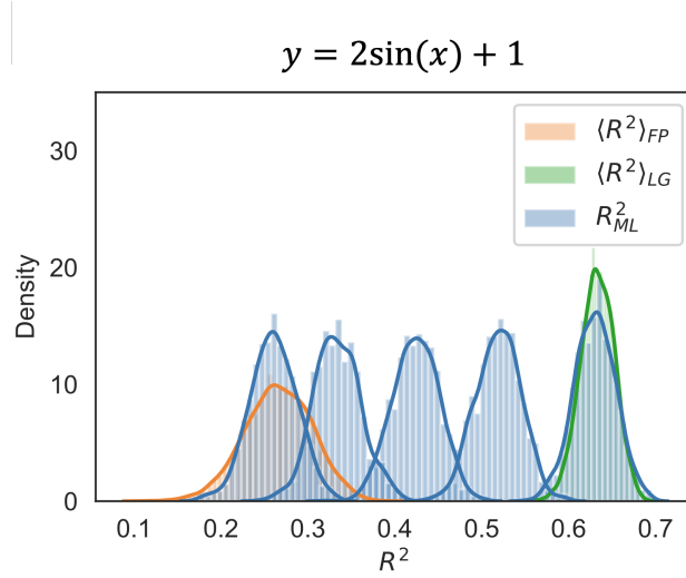
Figure 21. R^2 by assuming different levels of feature noise for the dataset generated by a nonlinear function y = 2\sin(x) + 1 + \varepsilon . Since x and \varepsilon are normally distributed, the nonlinear transformation gives a non-normally distributed \{y_{obs,i}\} .
