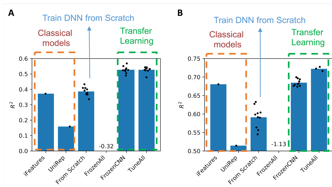
Figure 24. R^2 score of ML models on hold out test datasets. (A) Enzyme T_{\text{opt}} dataset; (B) Protein T_{\text{m}} dataset.
