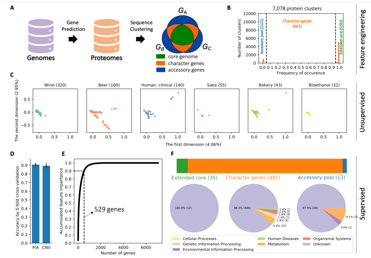
Figure 6. Resolving yeast GPR with pan-genome and ML. (A) The pan-genome reconstruction process. (B) Histogram chart that describes the distribution of the fraction of strains that each gene cluster covers. Those gene clusters were manually categorized into three groups: extended core (gene clusters that cover at least 95% of strains), accessory pool (gene clusters that cover only 5% or less of strains) and character genes (genes that cover 5–95% of strains). The number of gene clusters belonging to each category was shown in the parentheses. (C) Multiple correspondence analysis on the presence/absence of genes in the pan-genome. (D) Accuracy score obtained by 5-fold cross-validation with a random forest classifier using gene P/A or CNV features. (E) Accumulated feature importance curve from (D) on P/A dataset. The top genes contribute to 90% of the prediction power. (F) The pan-genome categories and KEGG function categories of the top genes.
