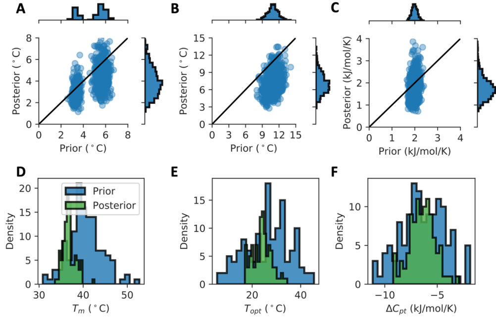
Figure 14. Large uncertainties in the Posterior etcGEM. (ABC) Parity plots of updated standard variance of enzyme (A) T_m s, (B) T_{opt} s, and (C) \Delta C_p^\ddagger s. (DEF) Prior and Posterior distributions of those three parameters of enzyme ERG1.
