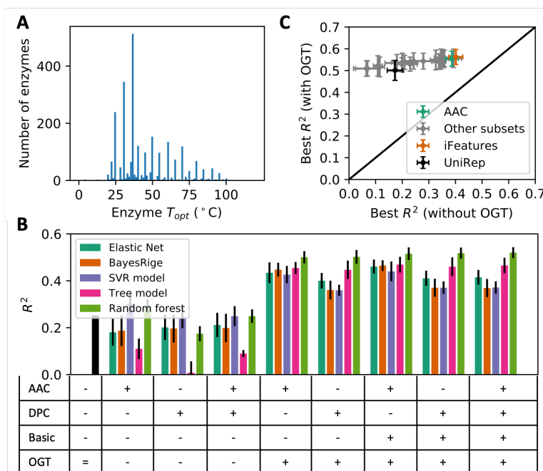
Figure 9. Development of enzyme T_{\text{opt}} prediction model. (A) Distribution of T_{\text{opt}} values in the training dataset. (B) 5-fold cross-validation results for five regression models on different feature sets. The “=” shows the explained variance when using OGT as the estimation of enzyme T_{\text{opt}} . “+” and “-” denote the presence and absence of feature sets used for ML analysis. Error bars show the standard deviation of R^2 scores obtained in 5-fold cross validation. AAC, amino acid frequencies; DPC, dipeptide composition; Basic, basic properties of proteins. (C) The performance comparison between the best regression models on different feature sets with and without OGT as an additional feature.
