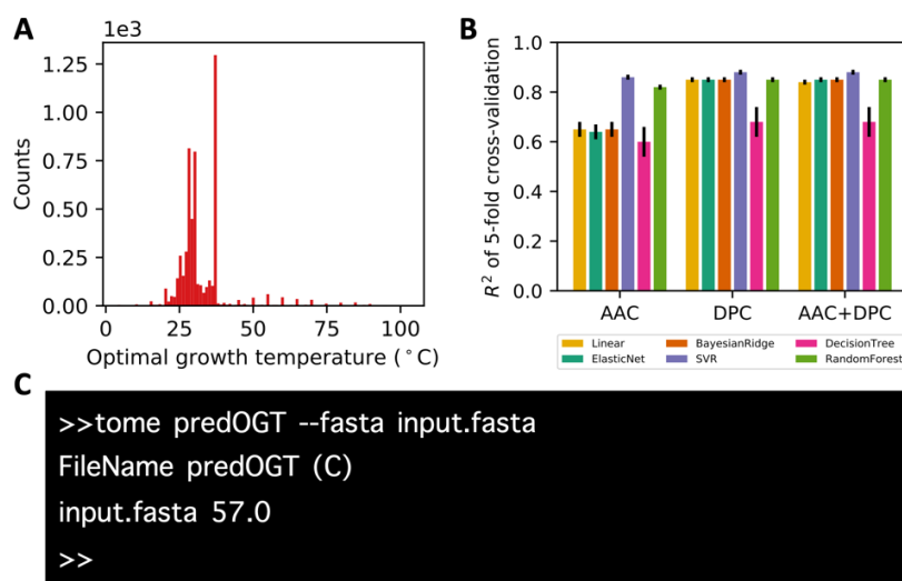
Figure 7. Development and release of OGT prediction model. (A) Distribution of OGTs in the training dataset; (B) Coefficient of determination score ( R^2 ) obtained by a 5-fold cross-validation for six different regression models. Error bars represent the standard deviation of R^2 scores. AAC, amino acid composition; DPC, dipeptide composition; (C) A command line tool (Tome) for OGT prediction was developed.
