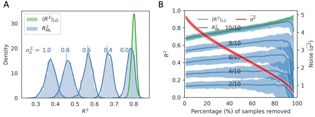
Figure 18 Monte Carlo simulations on (A) R^2 by assuming different levels of feature noise (a linear real function y = 2x + 1 was used); and (B) data cleaning via gradually removing the samples with the largest \sigma_{y,i} . n/10 indicate that n features out of a complete set of 10 features are used to train and validate the model. Noise values are given as the average variance of all samples ( \overline{\sigma_y^2} ). A linear real function f(x) = \sum_{i=1}^{10} x_i was used.
