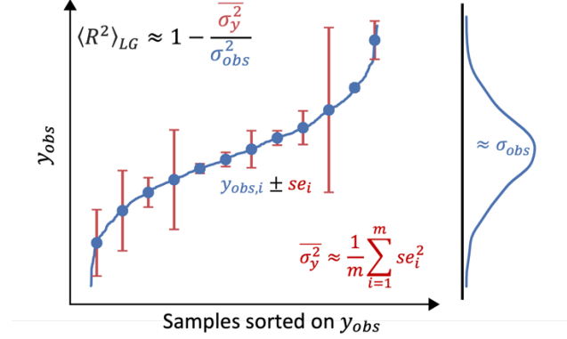
Figure 17. Schematic diagram depicting the estimation of the upper bound of model performance \langle R^2 \rangle_{LG} based on experimental label noise. Data shown were randomly generated, se_i denotes standard error of sample i .
