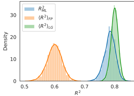
Figure 16. Monte Carlo simulation on the upper bound of R^2 . A linear real function y = 2x + 1 was used.
