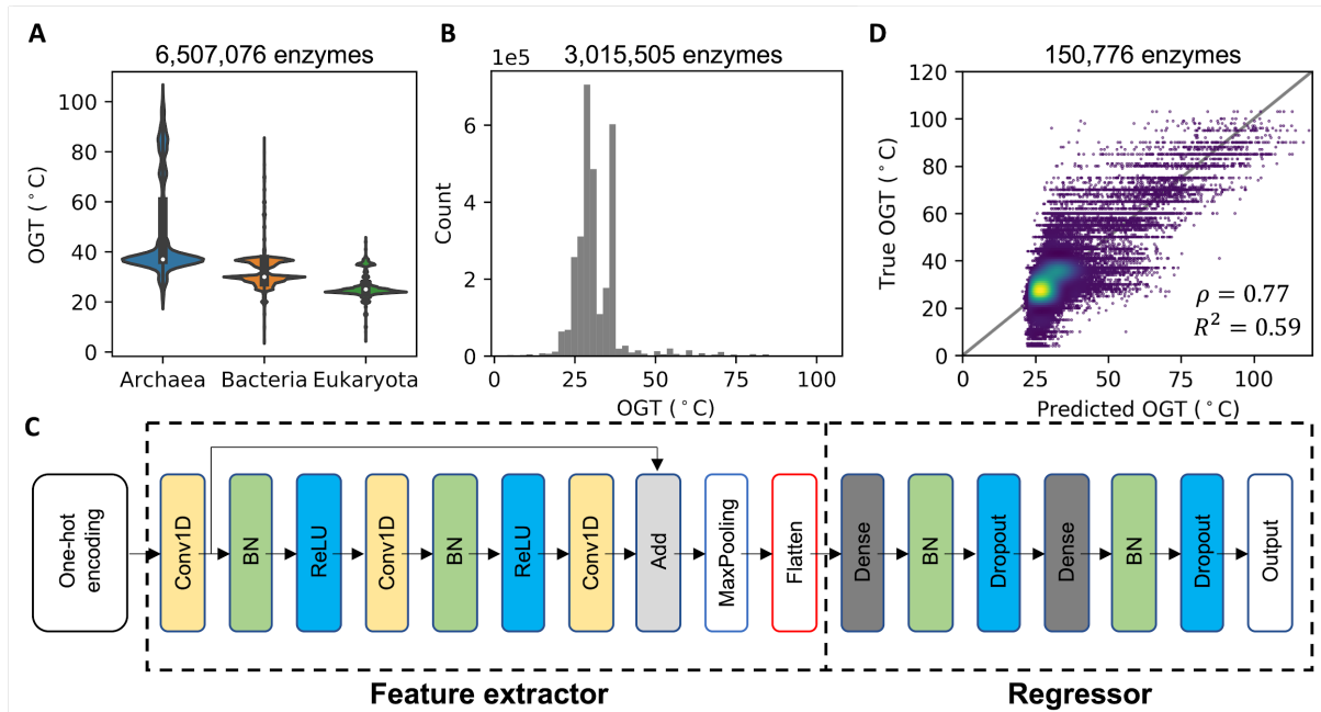
Figure 23. Pre-training with enzyme sequences labeled with OGT. (A) Violin plot of distributions of OGT-annotated enzymes from microorganisms belonging to three domains. (B) Distribution of OGT values after filtering out low-quality and redundant sequences. (C) The ResNet architecture used. (D) The comparison between predicted and true OGT values of enzymes in the hold out test dataset. \rho denotes Pearson's correlation coefficient and R^2 denotes the coefficient of determination.
