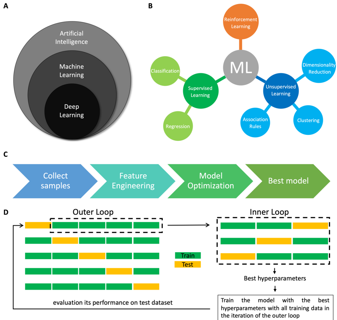
Figure 3. Machine learning. (A) Relationships between Artificial Intelligence (AI), Machine Learning (ML) and Deep Learning (DL). (B) Different categories of ML problems. (C) General steps for the development of a ML model. (D) An illustration of nested cross-validation approach. 5-fold for the outer loop and 3-fold for the inner loop are shown.
