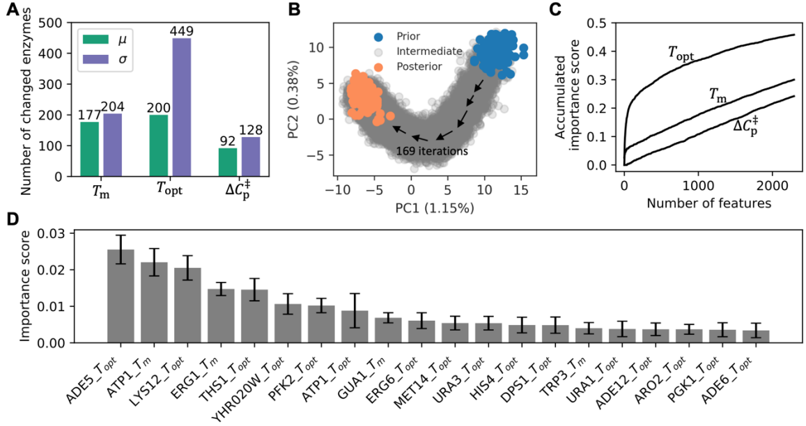
Figure 13. (A) The number of enzymes with a significantly changed mean and variance in T_m , T_{opt} and \Delta C_p^\ddagger between Prior and Posterior . (B) PCA on 21,504 parameter sets ( \hat{\theta} ) sampled in the SMC-ABC. (C) The accumulated importance score from the random forest model for each of the three parameter categories. (D) The top 20 parameters with the highest importance score were shown.
