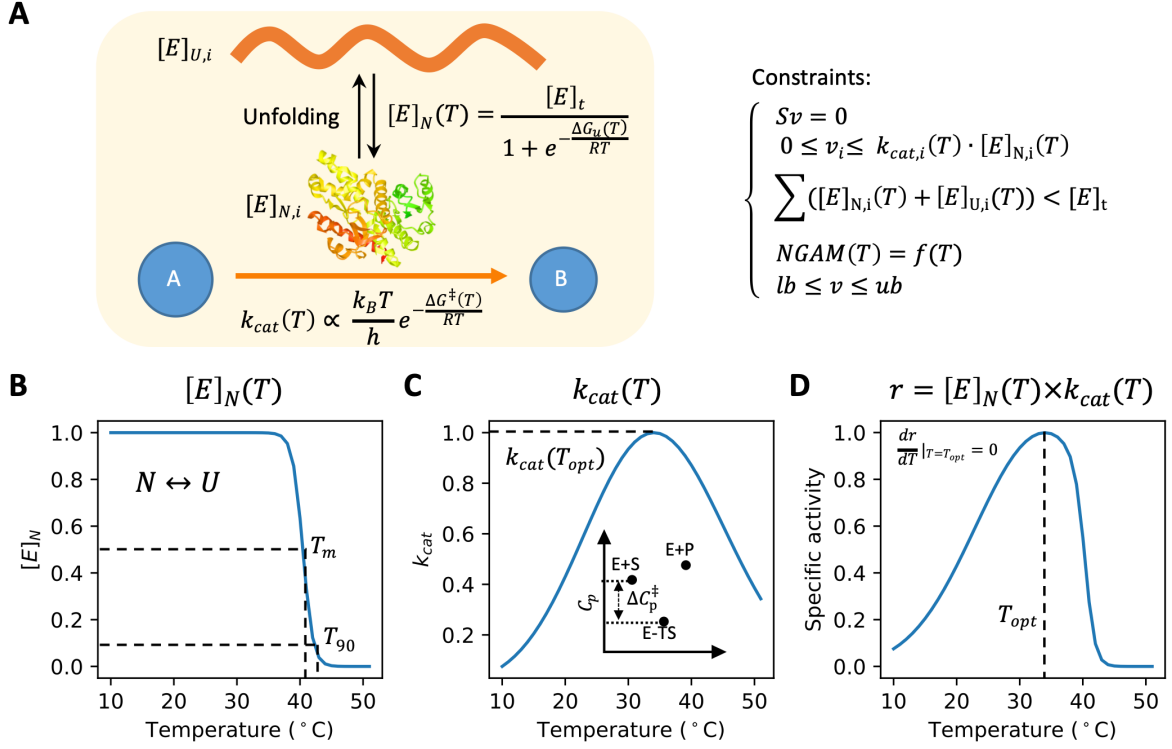
Figure 8. Enzyme and temperature constrained GEM (etcGEM). (A) An illustration of the temperature effects on enzyme-catalyzed reactions and their integration into a constrained GEM. (B) A two-state denaturation model was used to describe the temperature dependent unfolding process. [E]_N is the concentration of the enzyme in native state; T_{opt} is the optimal temperature at which the specific activity is maximized; T_m and T_{90} are temperatures at which there is a 50% and 90% probability that an enzyme is in the denatured state, respectively. (C) Macromolecular rate theory describing the temperature dependence of enzyme turnover number k_{cat} . Inset shows the heat capacity difference between ground state (E+S) and transition state (E-TS), adapted from Hobbs J., et al (Hobbs et al., 2017). (D) Temperature dependence of enzyme specific activity r , which is a product of (B) and (C).
