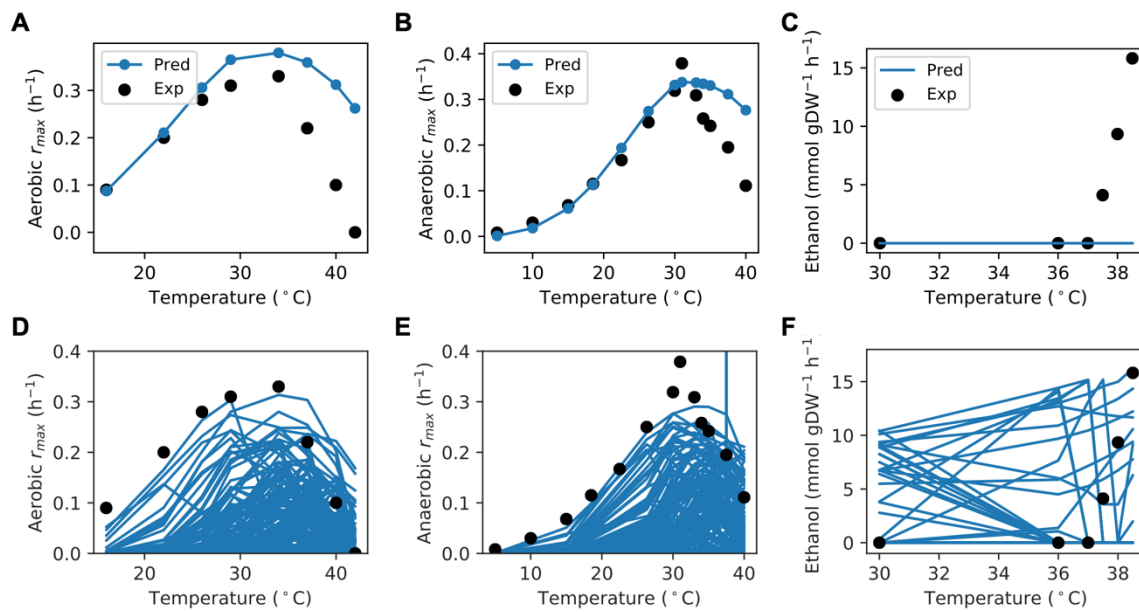
Figure 11 Simulated results of specific growth rate at (a) aerobic, (b) anaerobic batch cultivations and (c) ethanol flux at chemostat cultivation with etcGEM at different temperatures. Pred, predicted results by etcGEM. Exp, experimental data. (DEF) Simulated results when randomly sampling parameters (128 times) from pre-defined distributions that describe the uncertainties in the parameter values. r_{max} , maximal specific growth rate, corresponding to the y-axis label in A and B.
