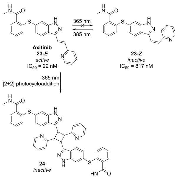
Figure 18. Photoinduced isomerisation of known VEGFR2 inhibitor Axitinib (23-Z→23-E) upon exposure to 385 nm, as well as the [2+2] photocycloaddition of 23-E to 24 when irradiated with light of wavelength 365 nm.
