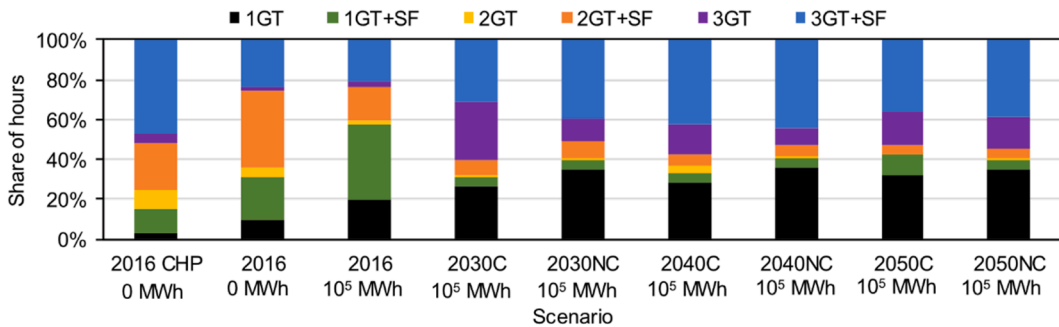
Fig. C.2. Optimal utilization of gas turbines and supplementary firing for the 2016–2050 scenarios. CHP = operation without product flexibility. The thermal flexibility available is given in MWh.
