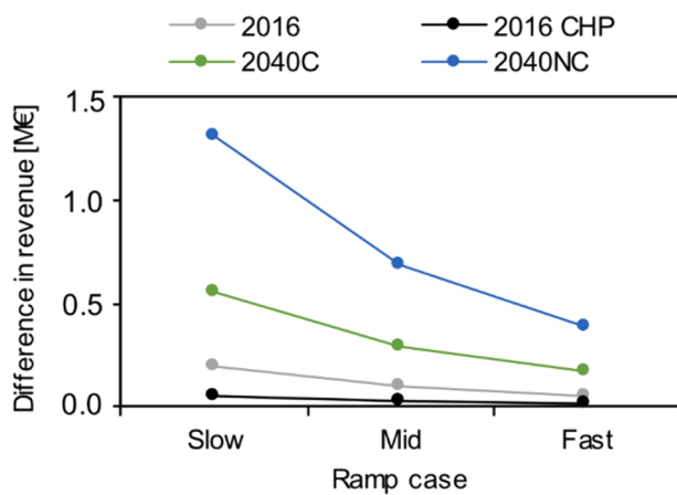
Fig. 18. Estimated annual difference in revenue, comparing static and dynamic plant operation for four electricity price scenarios. Thermal and product flexibilities are available except in 2016 CHP (no product or thermal flexibility). The exact values are given in Appendix D.
