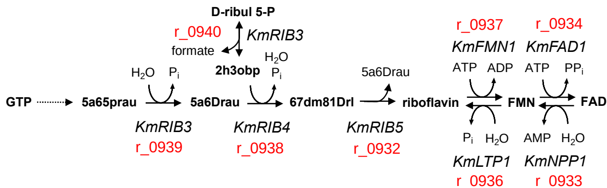
Figure 17. The riboflavin biosynthetic pathway. The gene names are written in italic, while the iSM996 reaction IDs are written in red colour. Abbreviations for metabolites: GTP (guanosine-5'-triphosphate), 5a65prau (5-amino-6-(5-phosphoribitylamino)uracil), 5a6Drau (5-amino-6-(D-ribitylamino)uracil), D-ribul 5-P (D-ribulose 5-phosphate), 2h3obp (2-hydroxy-3-oxobutyl phosphate), 67dm81Drl (6,7-dimethyl-8-(1-D-ribityl)lumazine production). Abbreviations for genes: KmRIB3 (3,4-dihydroxy-2-butanone-4-phosphate synthase), KmRIB4 (lumazine synthase), KmRIB5 (riboflavin synthase), KmFMN1 (riboflavin kinase), KmFAD1 (FAD synthetase), KmLTP1 (putative protein phosphotyrosine phosphatase), KmNPP1 (nucleotide pyrophosphatase/phosphodiesterase).
