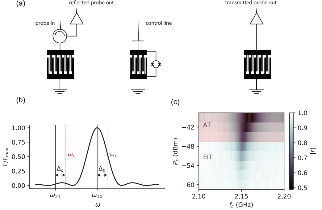
Figure 3.3: a) Device schematic. The delayline consists of two IDTs with 150 finger pairs separated by a distance of 400 μm. It is used to probe the SAW reflection and transmission of the transmon qubit, which has 25 finger pairs and a capacitively coupled gate electrode where the control signal is applied. b) Frequency dependence of the acoustic coupling strength with annotations for the probe and control tone frequencies as well as the transmon transition frequencies. c) Probe reflection measured as a function of control frequency and power of the signal applied at room temperature. In the red shaded region the control tone strength \Omega_c > 16 MHz and the transparency is due to the AT splitting. For weaker control tones EIT is observed.
