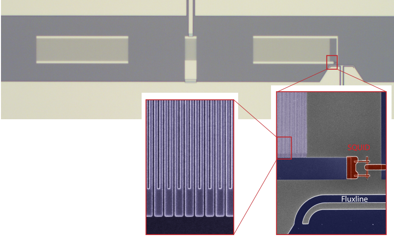
Figure 5.2: Microscope image of the QUAKE device used in experiments. The edges of the Bragg mirrors are separated by L_e = 600 \mu\text{m} . The SQUID mirror on the right hand side has 500 periods (1000) fingers. The sample is fabricated from aluminium on a gallium arsenide substrate. Insets show false-colour scanning electron micrographs of the SQUID, fluxline, and finger structure.
