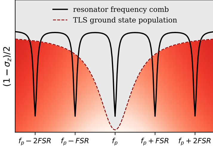
Figure 4.3: Illustration of TLS spectral hole burning in a multimode SAW resonator. The black line shows the comb structure of the SAW modes, spaced by the free spectral range. The ground state population of the TLS ensemble is plotted as a function of detuning from the pump mode (red dashed line and colourscale). A higher unsaturated TLS density within the linewidth of a mode implies more loss, and the effect of the pump is to burn a "hole" in the absorption spectrum of the TLS distribution. Increasing the power of the pump tone will saturate more TLSs cause the width of the spectral hole to widen.
