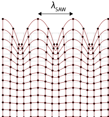
Figure 1.1: Illustration of a Rayleigh wave in the plane of propagation. The Rayleigh mode is a superposition of longitudinal and transversal modes, leading to elliptical particle trajectories with a vertical major axis. The amplitude of the excitation decays exponentially into the bulk of the material with a depth approximately corresponding to the wavelength \lambda_{\text{SAW}} . The displacements have been greatly exaggerated for illustration.
