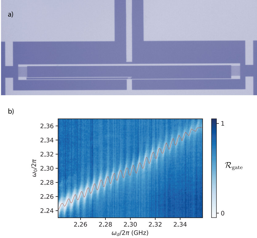
Figure 3.9: a) Microscope image of a giant atom device of length L = 550 \mu\text{m} with an electrical gate. b) Gate reflection (normalized) measured with a vector network analyser for a giant atom of the design depicted in a) . The modulation of the effective maximal transduction frequency is highlighted by the red line. Towards the edges of the frequency range, the modulation amplitude starts to diminish due to the limited bandwidth of the local coupling point IDTs.
