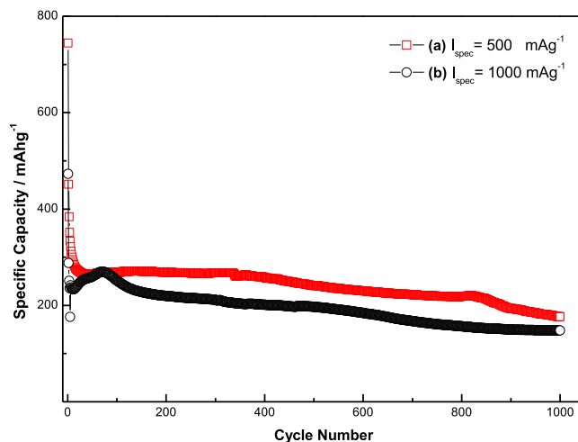
Figure 7. Extended galvanostatic performance of \text{Fe}_3\text{O}_4/\text{C} cells comparison; 0.100 \text{ V} < E < 3.000 \text{ V} (a) I_{\text{spec}} = 500 \text{ mA g}^{-1} ; (b) I_{\text{spec}} = 1000 \text{ mA g}^{-1} .
