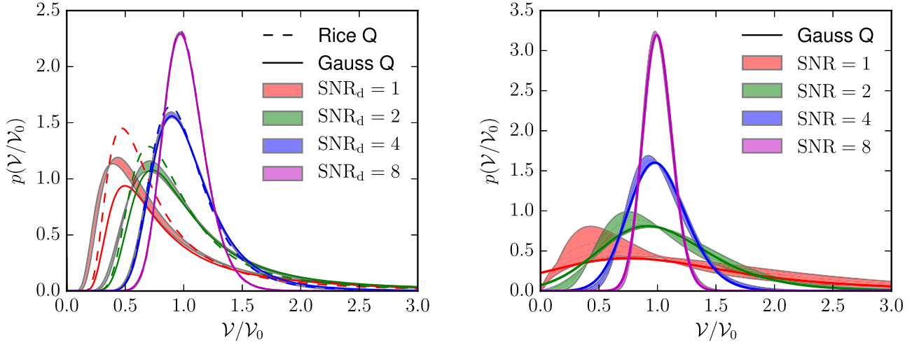
Figure B3. Left: comparison of the closure amplitude distribution with the Gauss Q approximation in Equation (B17) for various choices of the denominator S/N_d . In all cases, the numerator S/N was set to 8, divided equally among the visibility amplitudes in the numerator. For comparison, the visibility amplitude quotient (Rice Q ) distribution is also shown. The range of the filled bands indicates the uncertainty associated with various choices of how S/N_d is apportioned between the two visibility amplitudes in the denominator. In all cases, the value of \rho was set to the proper value in all models. Right: comparison of the closure amplitude distribution and the Gauss Q approximation with \rho = 1 , for \mathcal{V}_0 = 0.5 . The colored bands indicate the range of closure amplitude distributions when the true \rho is varied within the permissible range for the 2017 EHT campaign, [0.3,0.33]. The S/N within the numerator and denominator is distributed uniformly. Quantitative estimates of the accuracy of the various approximations for illustrative cases can be found in Table B4.
