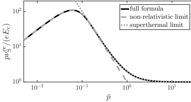
Figure 3.1: Dynamical friction force on an electron in a fully ionized plasma of temperature 1 keV (i.e. \Theta \approx 2 \cdot 10^{-3} ; \bar{p}_{\text{Te}} \approx 0.06 ), neglecting the energy-dependence of the Coulomb logarithm. The solid black line uses the full expression (2.13), whereas the gray lines show the limiting expressions (3.5). Note that radiation reaction also contribute to the energy loss at high energies, which means that the total friction on a relativistic electron increases with \bar{p} .
